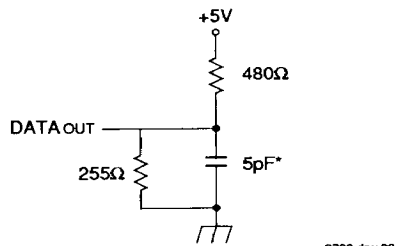
Figure 2. Output Load (for tRLZ, tWLZ, and tRHZ)
