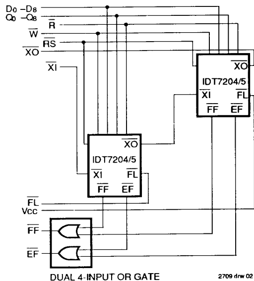
DUAL 4-INPUT OR GATE
