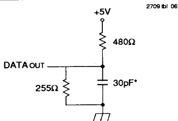
Figure 1. Output Load
