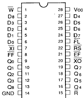
DSIP TOP VIEW
