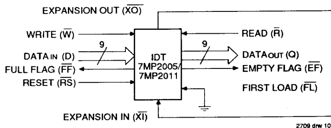
Figure 8. Block Diagram of Single IDT7MP2005/7MP2011 FIFO
