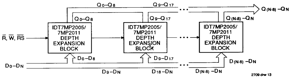
Figure 11. Compound FIFO Expansion
