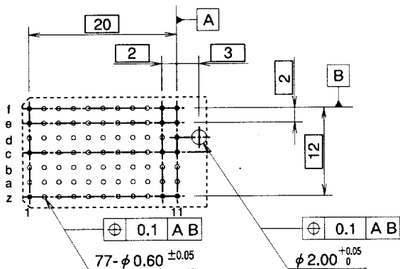
PCB Mounting dimensions (connector mount side)
