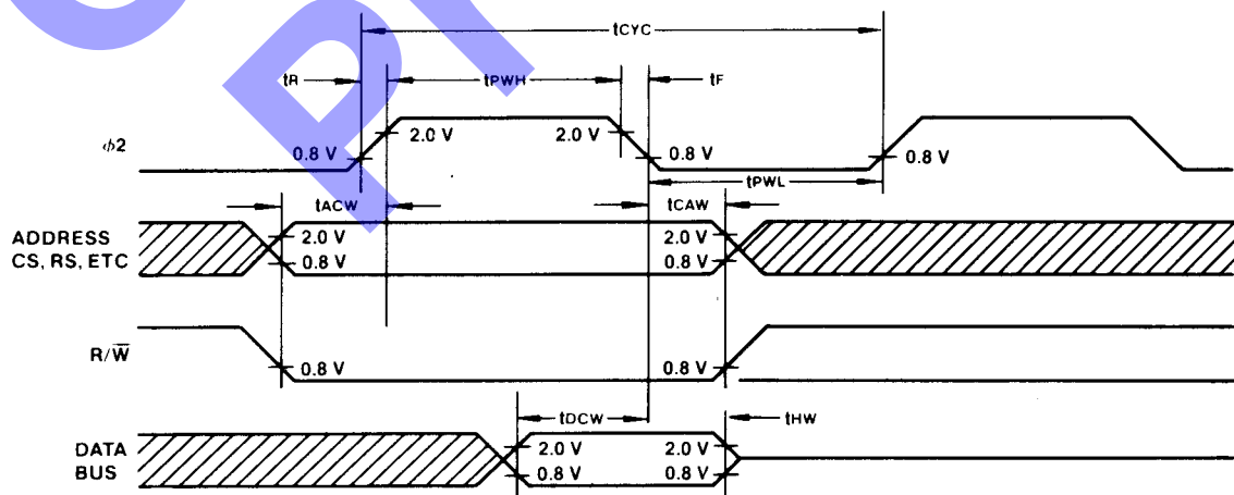
Figure 2. Write Timing
