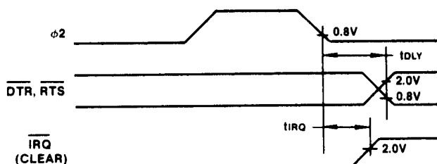
Figure 4. Interrupt and Output Timing
