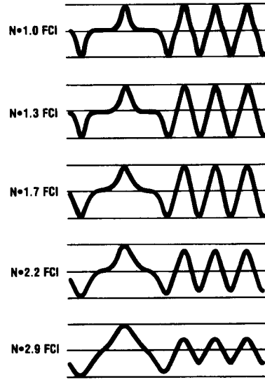
FIGURE 15. F-2.66 \times F Pulse Waveforms for Various Flux Changes per Inch
