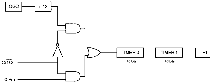
Figure 10.32 Bit Timer/counter.
