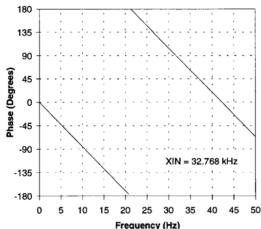
Figure 7. Filter Phase Plot to 50 Hz
