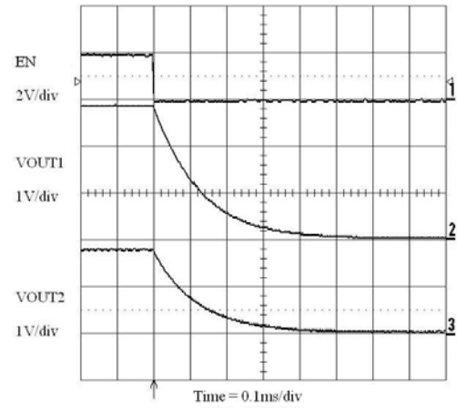
Figure 19. Enable Turn-off (100 μA Loads)
