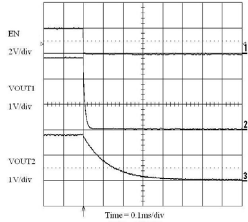
Figure 21. Enable Turn-off (300 mA/100 μA Loads)
