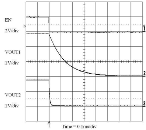
Figure 23. Enable Turn-off (100 μA/300 mA Loads)
