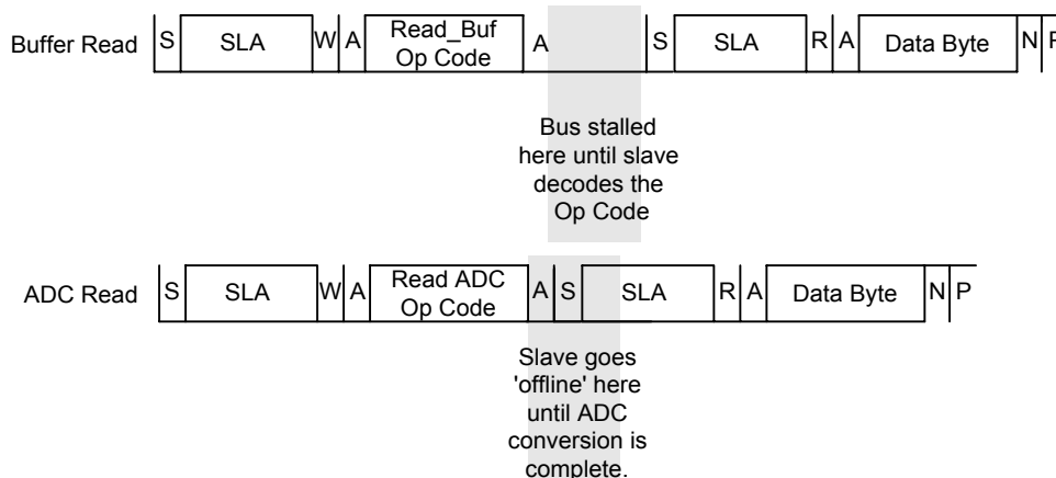
Figure 11. Peer-to-Peer Read Sequence
