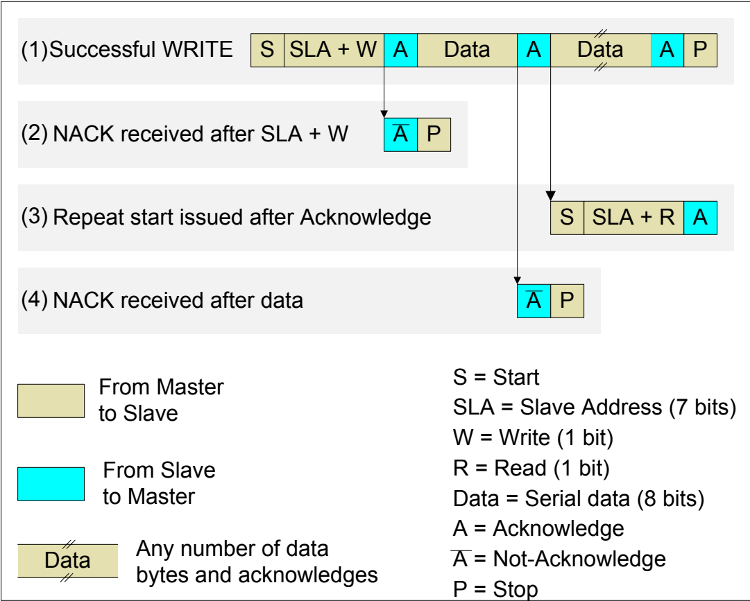
Figure 3. Typical WRITE Transfer Scenarios
