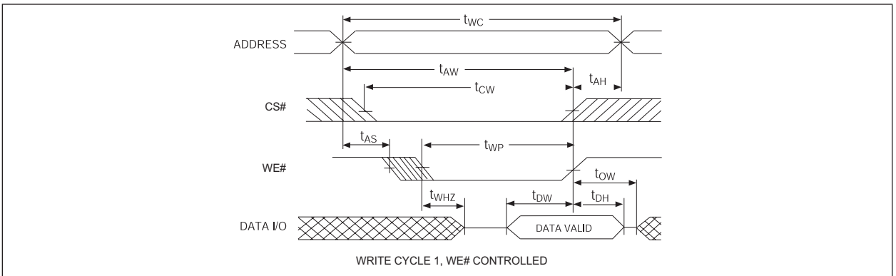
FIGURE 5 – WRITE CYCLE - WE# CONTROLLED
