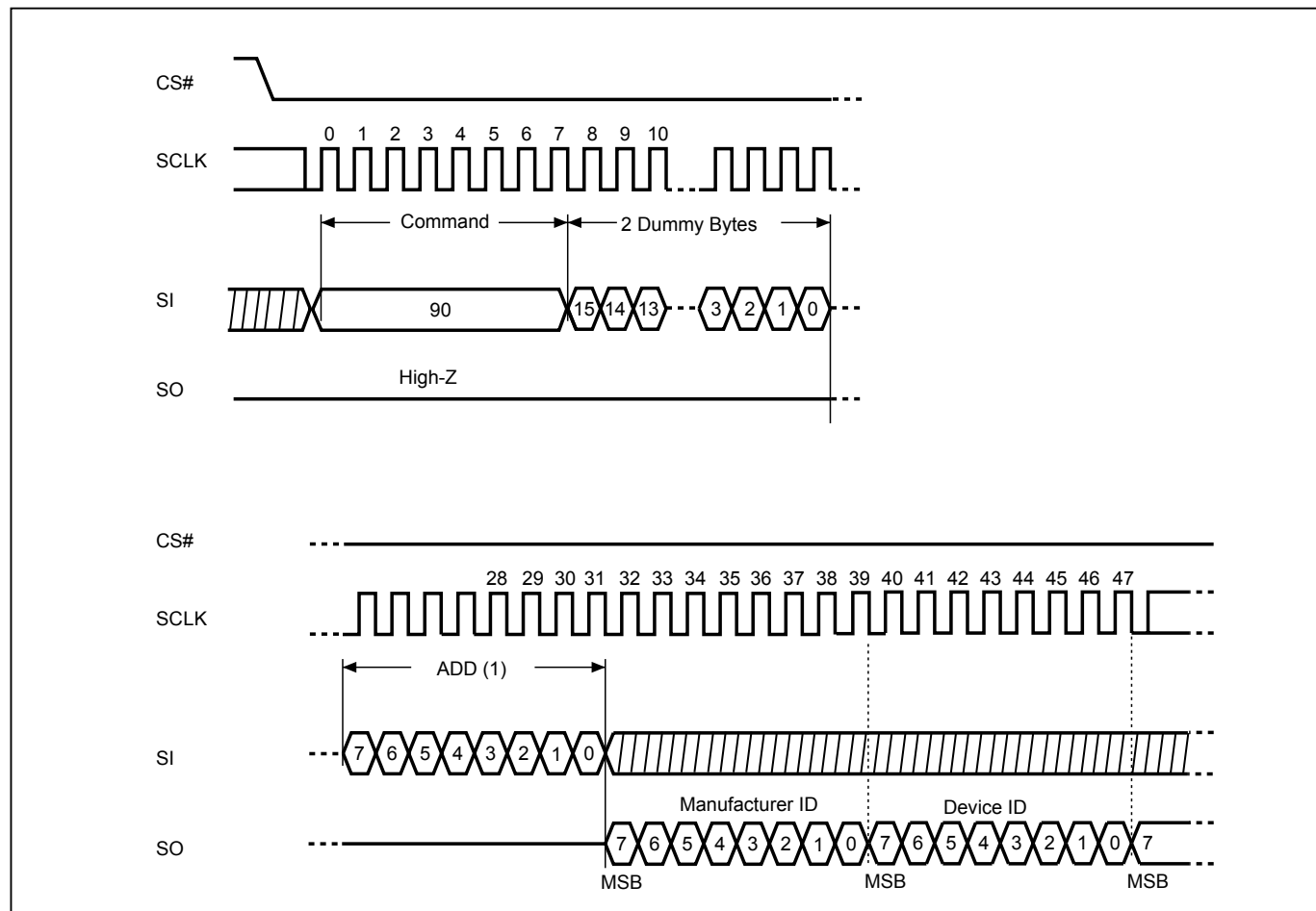
Figure 26. Read Electronic Manufacturer & Device ID (REMS) Sequence (Command 90 or EF)
