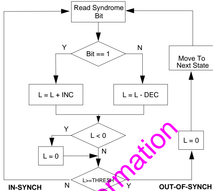
Figure 3-6. Synchronisation Flow
