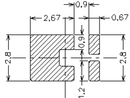
Soldering patterns
