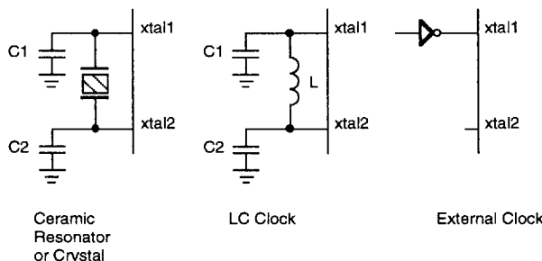
Figure 13. Oscillator Configuration
