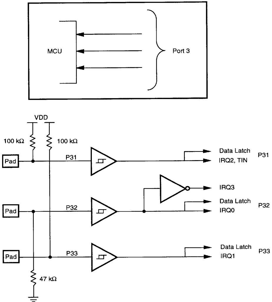
Figure 6. Port 3 Configuration
