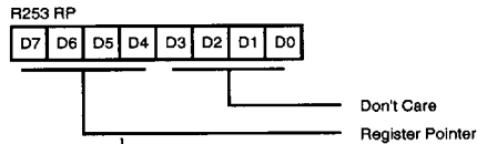
Figure 31. Register Pointer (FDH: Read/Write)
