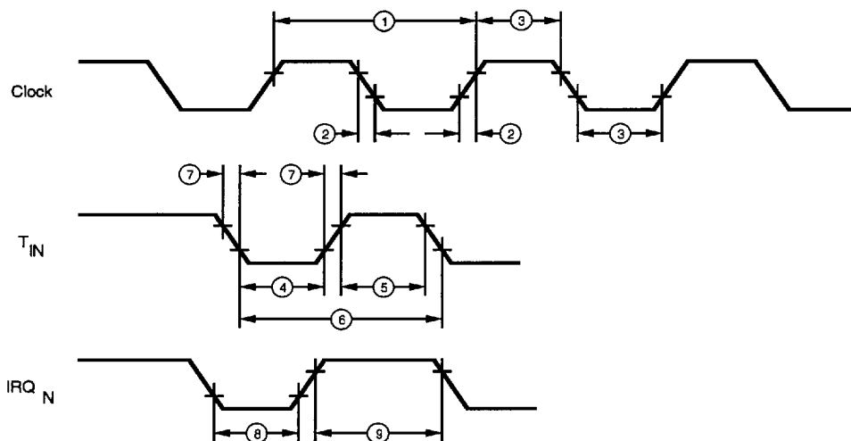
Figure 18. Electrical Timing Diagram
