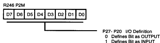
Figure 24. Port 2 Mode Register (F6H: Write Only)
