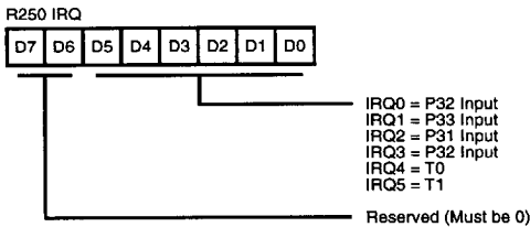
Figure 28. Interrupt Request Register (FAH: Read/Write)
