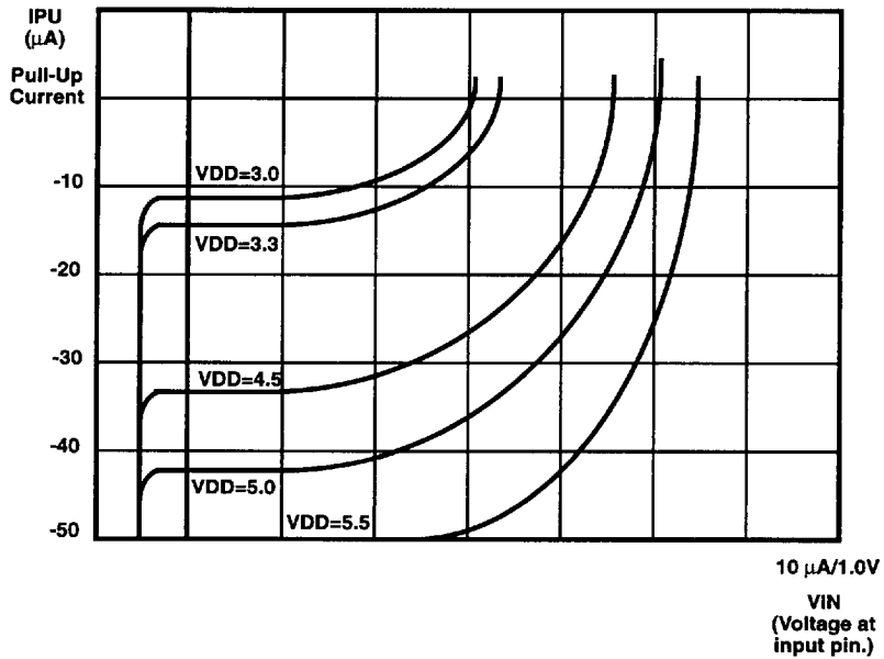
Figure 39. Pull-Up Resistance Characteristics Port P23-P20, P31, P33, P02-P00
