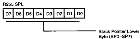
Figure 32. Stack Pointer (FFH: Read/Write)
