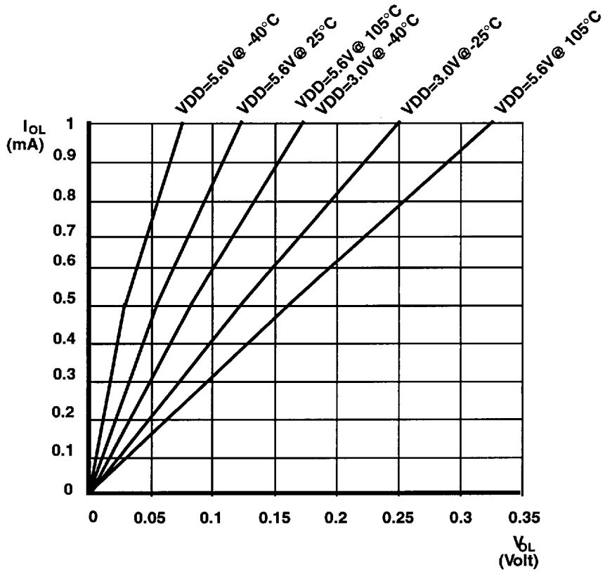
Figure 37. Typical I_{OL} vs V_{OL}
