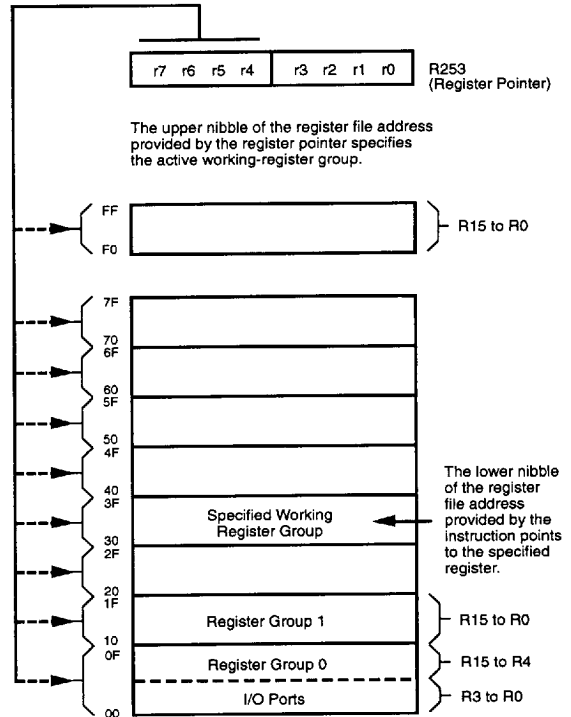
Figure 10. Register Pointer
