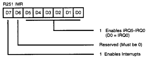
Figure 29. Interrupt Mask Register (FBH: Read/Write)
