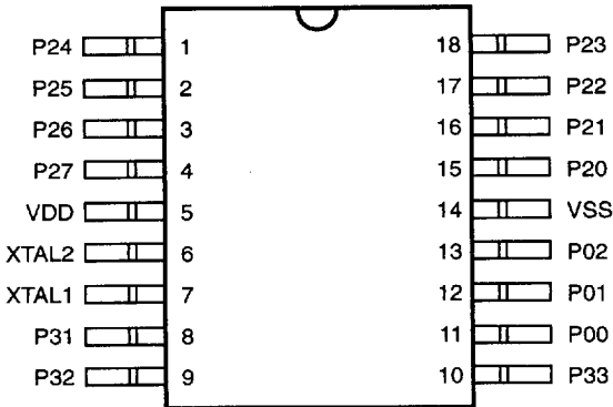
Figure 3. 18-Pin SOIC Pin Configuration
