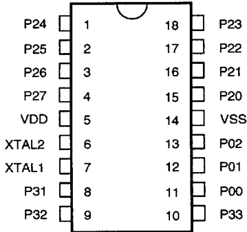
Figure 2. 18-Pin DIP Pin Configuration
