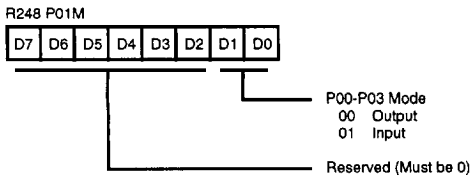
Figure 26. Port 0 and 1 Mode Register (F8H: Write Only)
