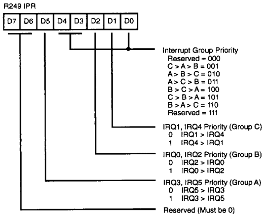
Figure 27. Interrupt Priority Register (F9H: Write Only)
