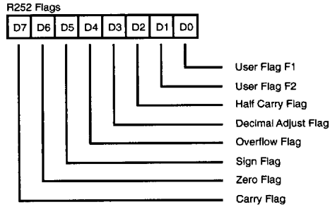
Figure 30. Flag Register (FCH: Read/Write)
