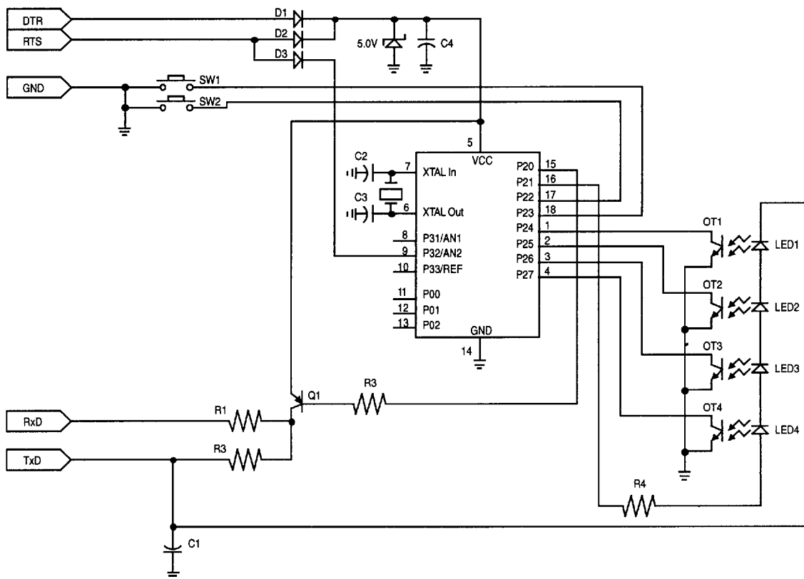
Figure 16. Circuit Diagram Of Z86C17 Two Button Mouse Application
