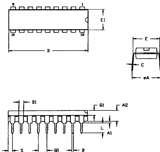
18-Pin Plastic DIP Package Diagram
