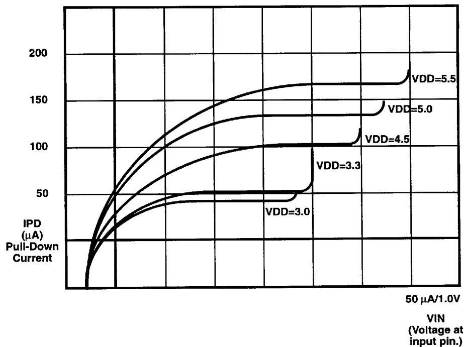
Figure 41. Pull-Down Resistance Characteristics Port P32
