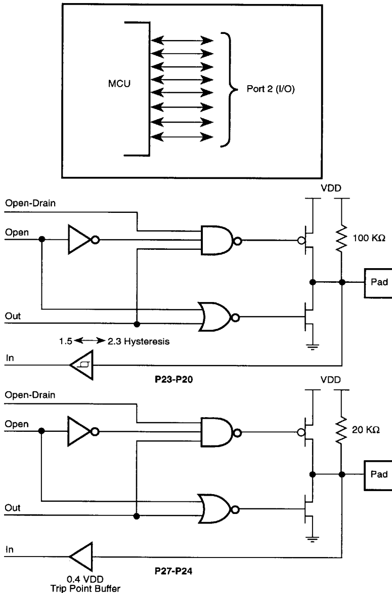
Figure 5. Port 2 Configuration
