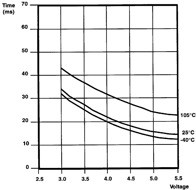
Figure 38. Typical WDT Time Out Period vs V_{DD} Over Temperature
