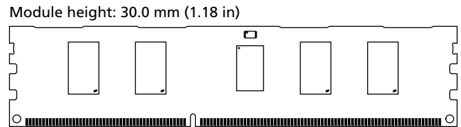
Figure 1: 240-Pin RDIMM (MO-269 R/C A)
