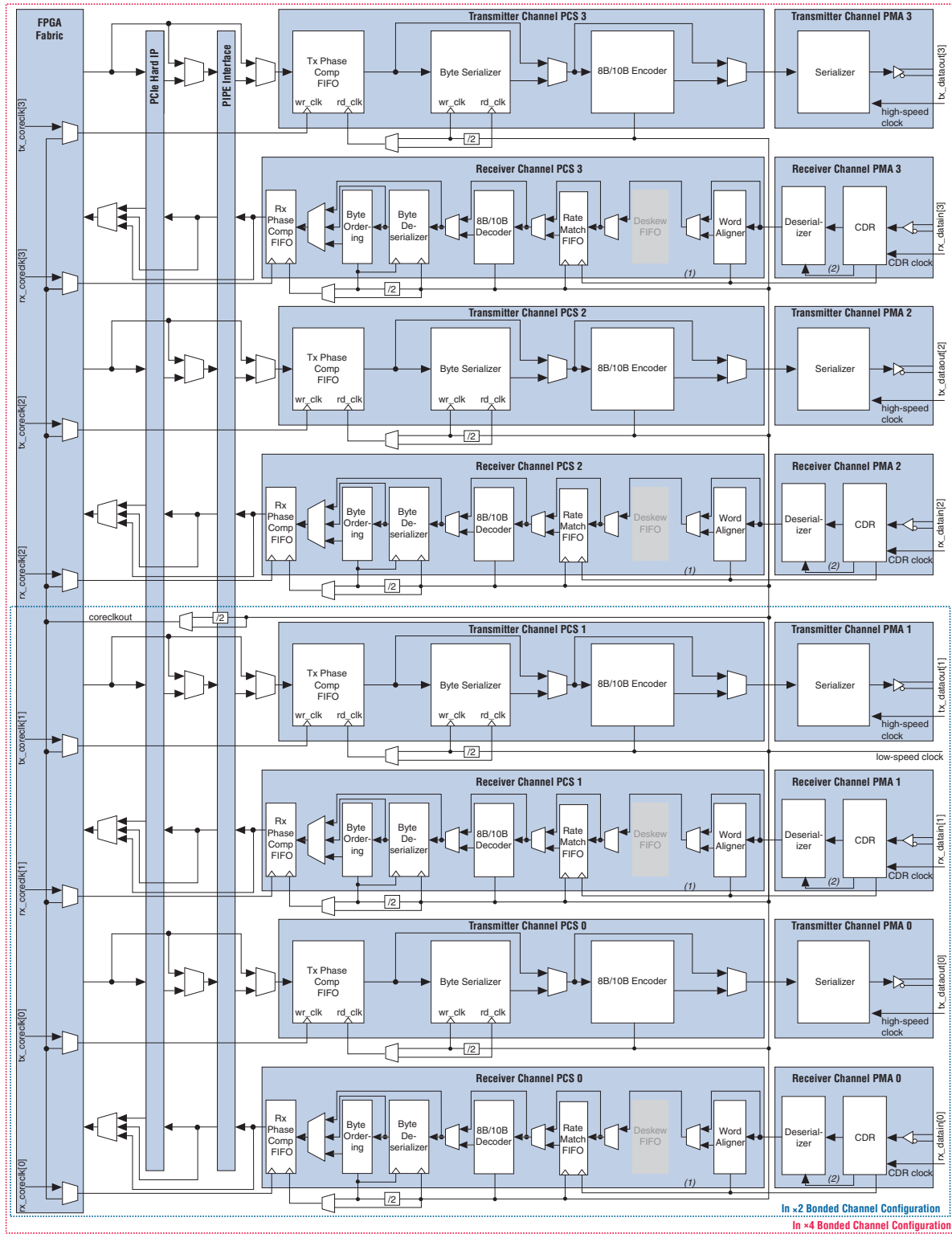
Figure 1-39. Transmitter and Receiver Datapath Cloning with Rate Match FIFO in Bonded Channel Configuration
