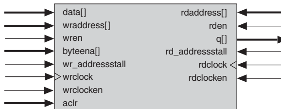
Figure 3-8. Cyclone IV Devices Simple Dual-Port Memory (Note 1)
