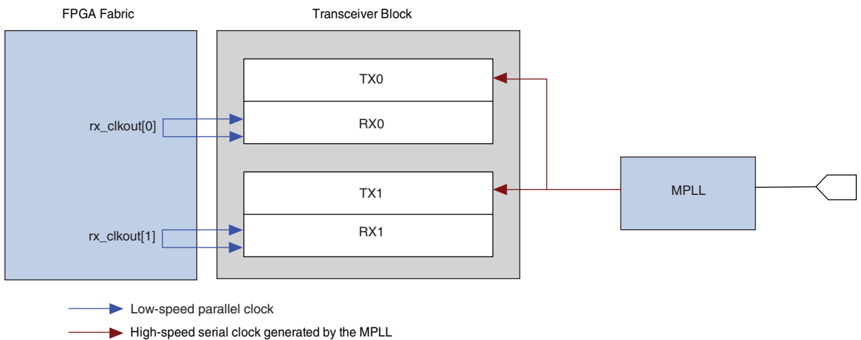
Figure 3–15. Option 3 for Receiver Core Clocking (Channel Reconfiguration Mode)
