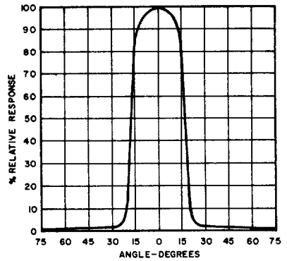
ANGULAR RESPONSE
