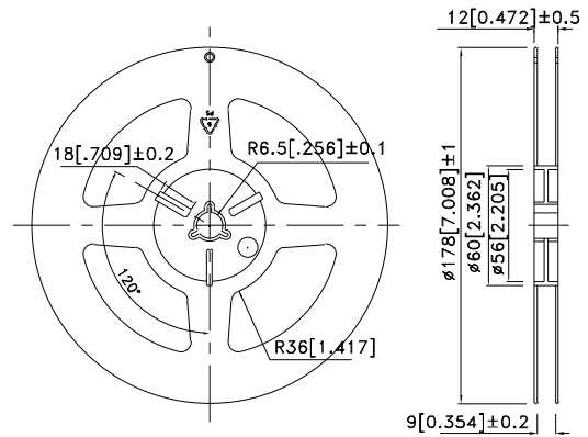
Reel Dimension
