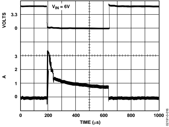
Figure 16. Short-Circuit Current
