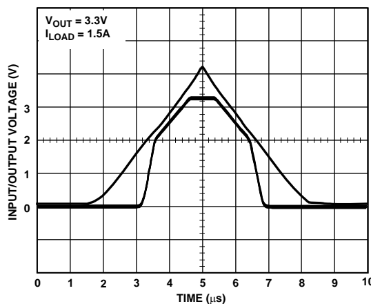
Figure 11. Power-Up/Power-Down
