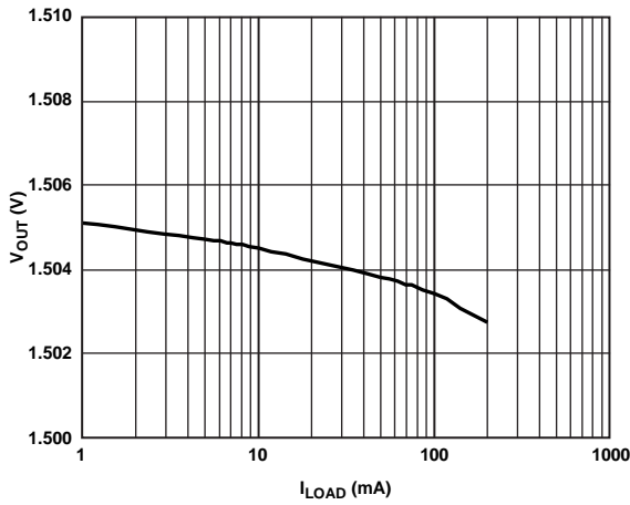
Figure 12. Output Voltage vs. Load Current
