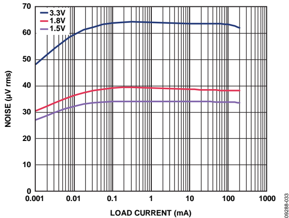
Figure 35. Output Noise vs. Load Current and Output Voltage, V_{IN} = 5\text{ V}
