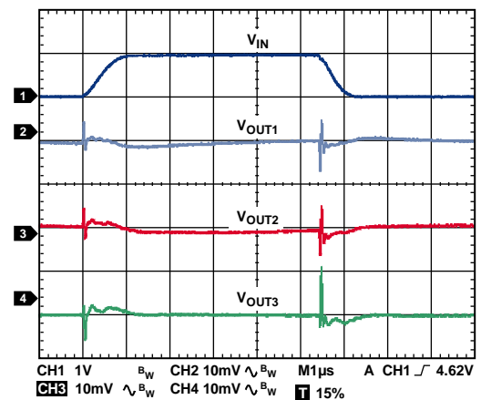
Figure 40. Line Transient Response, V_{IN} = 4\text{ V to } 5\text{ V} , I_{LOAD1} = I_{LOAD2} = I_{LOAD3} = 100\text{ mA} , CH1 = V_{IN} , CH2 = V_{OUT1} , CH3 = V_{OUT2} , CH4 = V_{OUT3}
