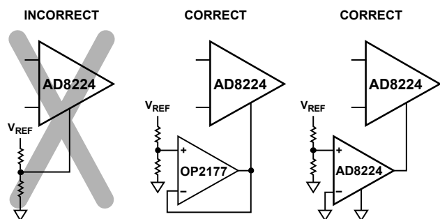
Figure 56. Driving the Reference Pin
