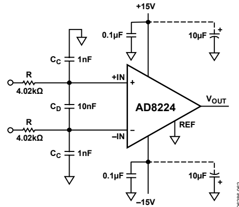
Figure 60. RFI Suppression
