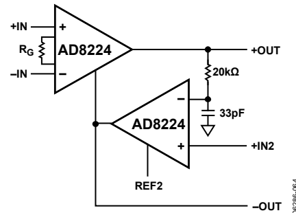
Figure 62. Differential Circuit Schematic
