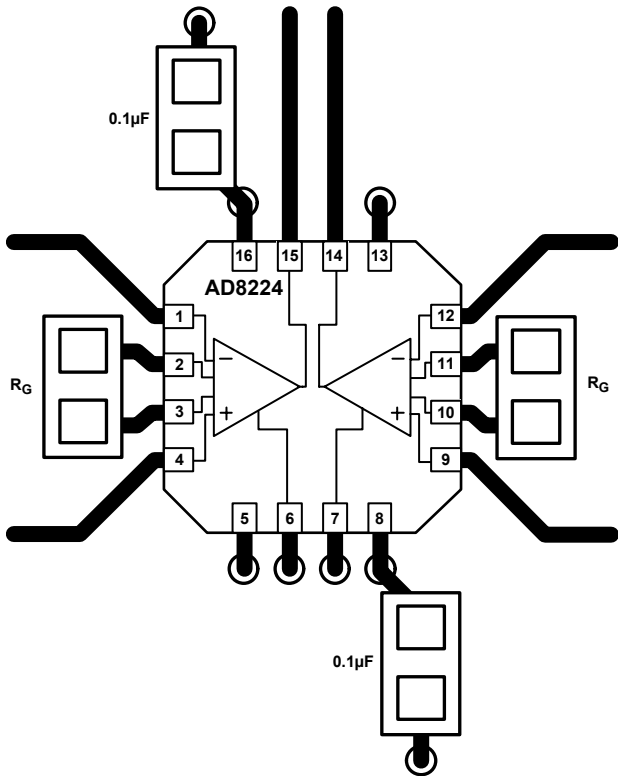
Figure 57. Example Layout
