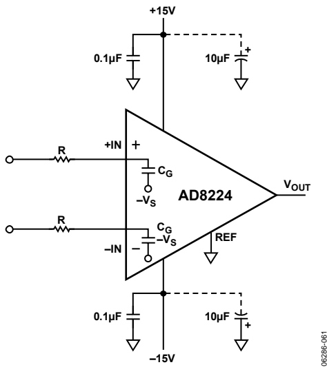
Figure 59. RFI Filtering Without External Capacitors
