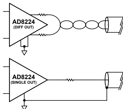
Figure 65. Driving a Cable
