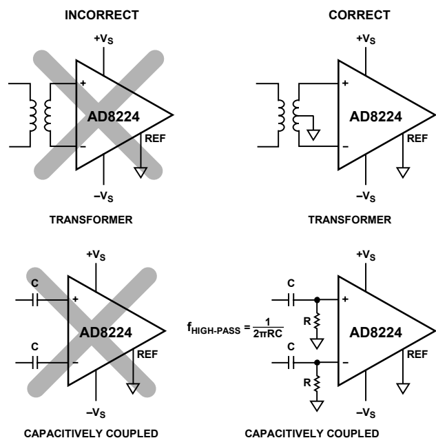
Figure 58. Creating an I_{BIAS} Path
