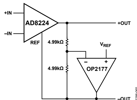
Figure 63. Differential Output Using Op Amp
