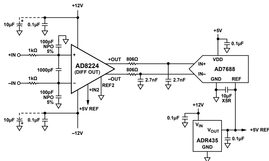
Figure 64. Driving a Differential ADC
