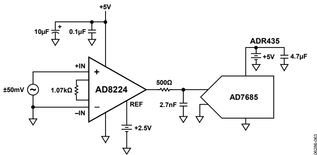
Figure 61. Driving an ADC in a Low Frequency Application
