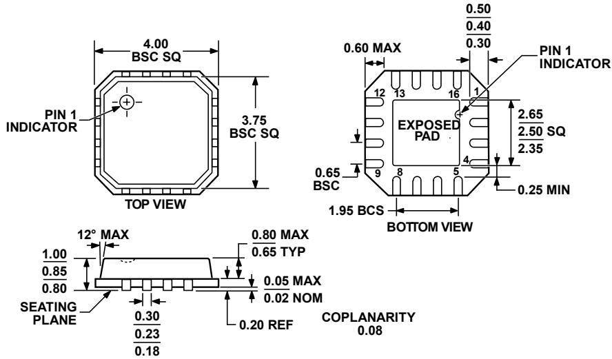
Figure 66. 16-Lead Lead Frame Chip Scale Package [LFCSP_VQ] 4 mm × 4 mm Body, Very Thin Quad (CP-16-13) Dimensions are shown in millimeters
