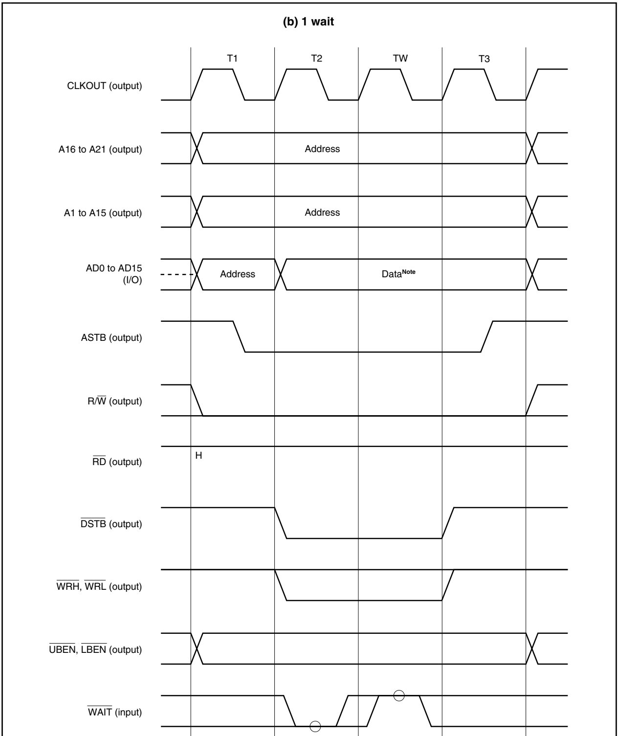
Figure 4-9. Memory Write (2/2)
