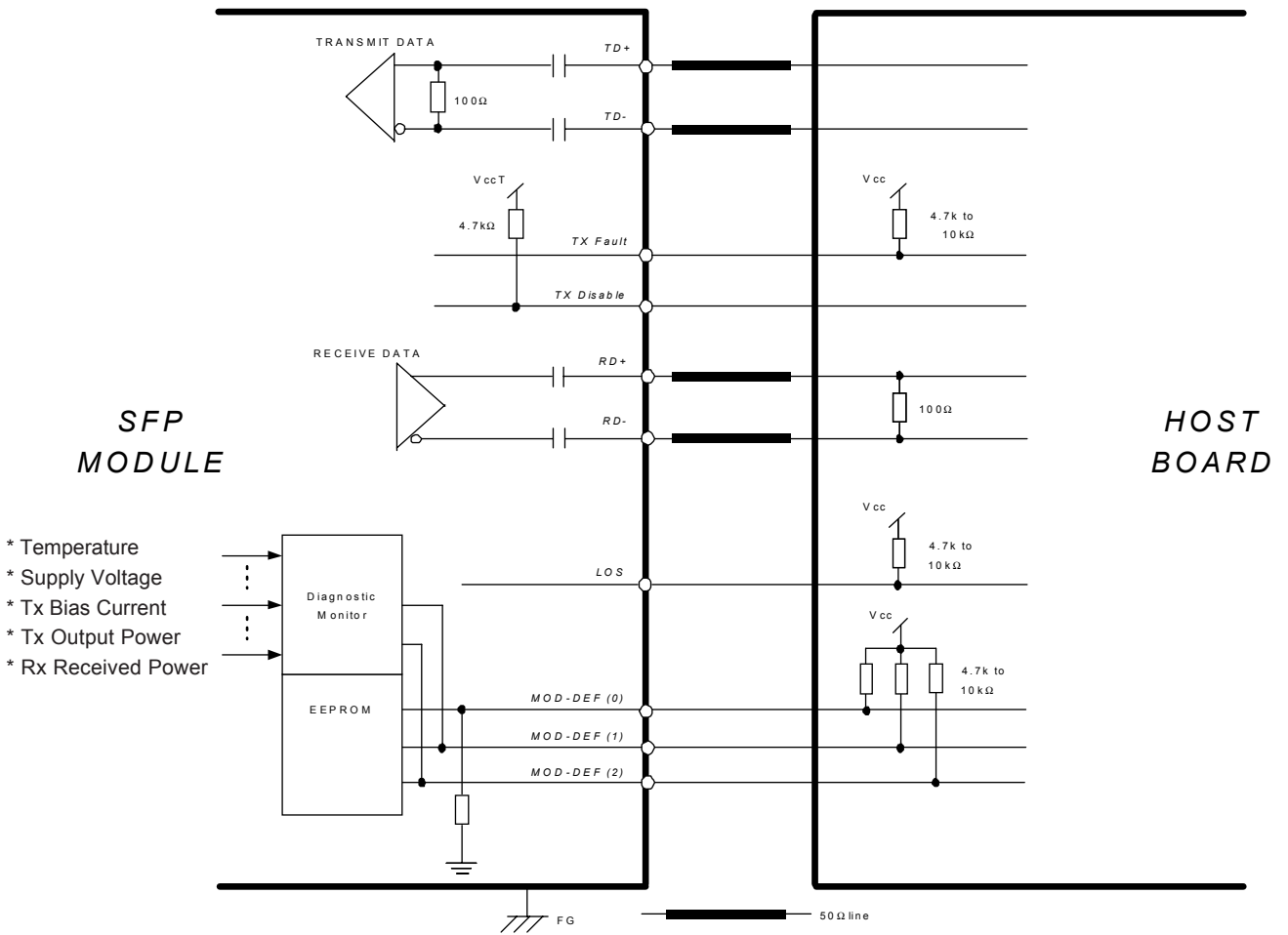
Figure 13. Recommended Interface Circuit (Diagnostic Monitor is incorporated for SCP6EN4-GL-#N-xx only.)
