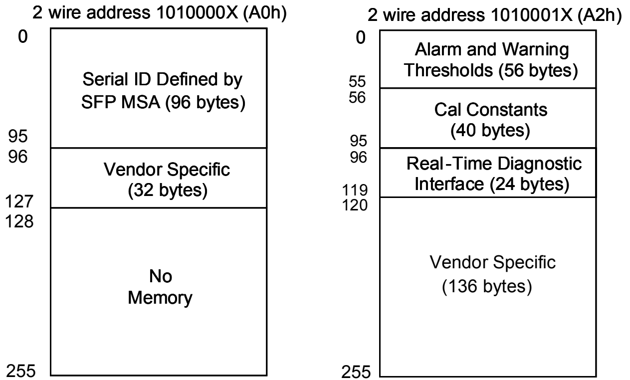
Figure 11. Digital Diagnostic Memory Map (A2h is applicable for SCP6EN4-GL-#N-xx)
