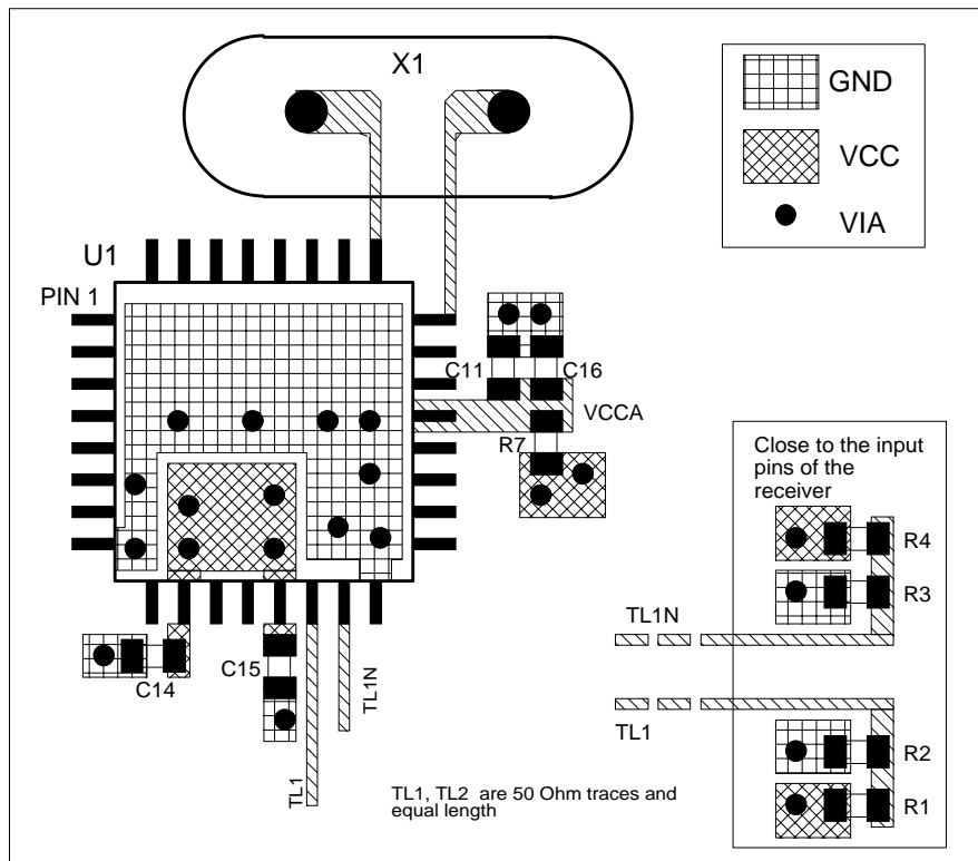
FIGURE 5B. PCB BOARD LAYOUT FOR ICS8430I-11
