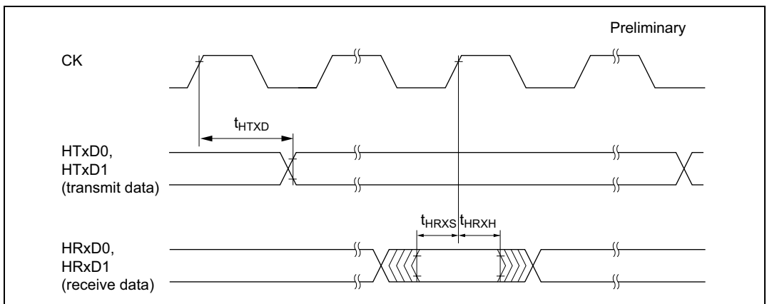
Figure 24-27 HCAN Input/Output Timing
