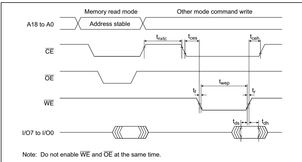
Figure 21B-19 Timing Waveforms in Transition from Memory Read Mode to Another Mode
