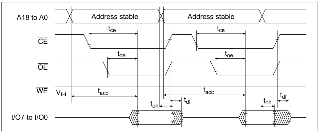
Figure 21C-21 \overline{\text{CE}} and \overline{\text{OE}} Clock System Read Timing Waveforms
