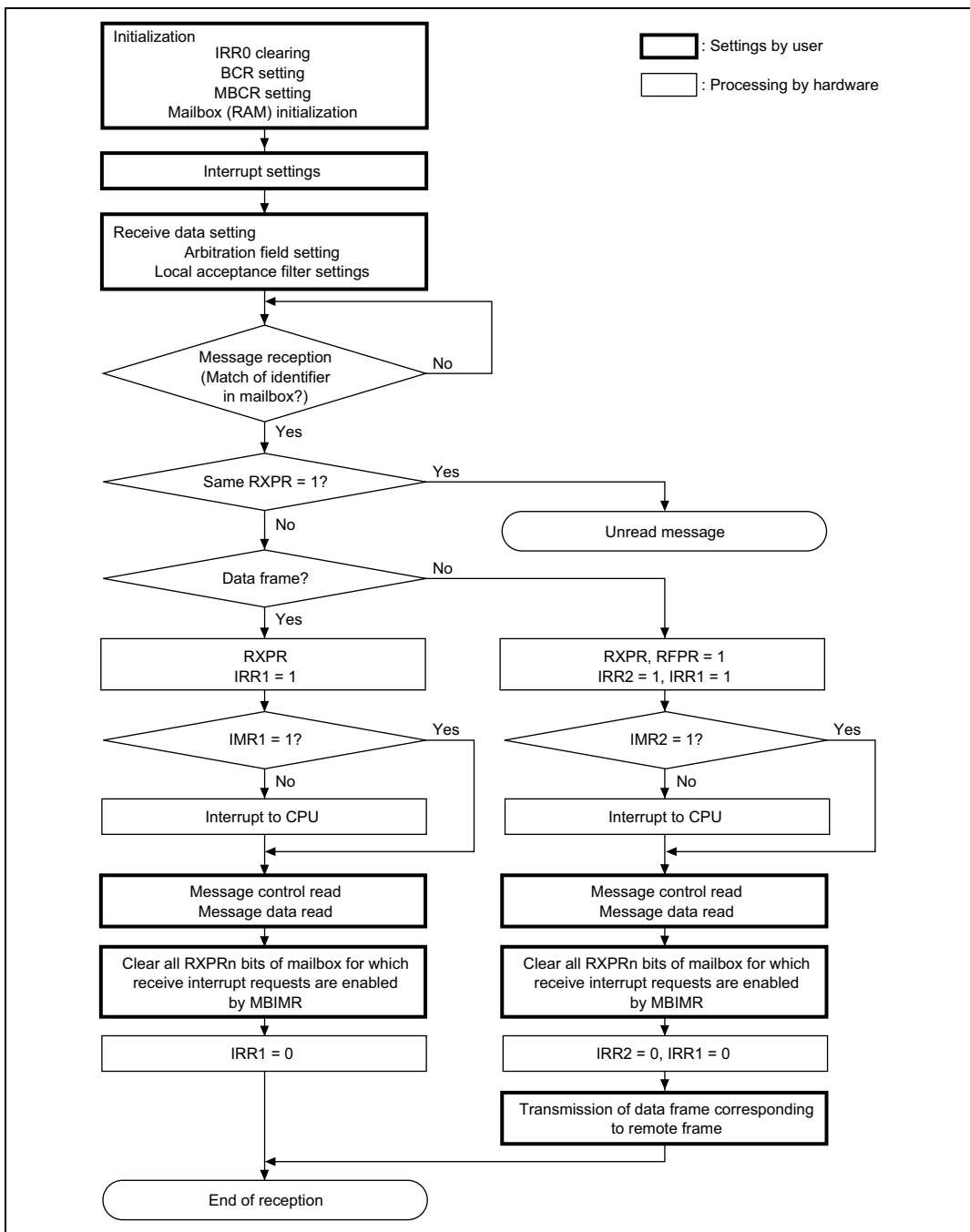
Figure 16-9 Reception Flowchart
