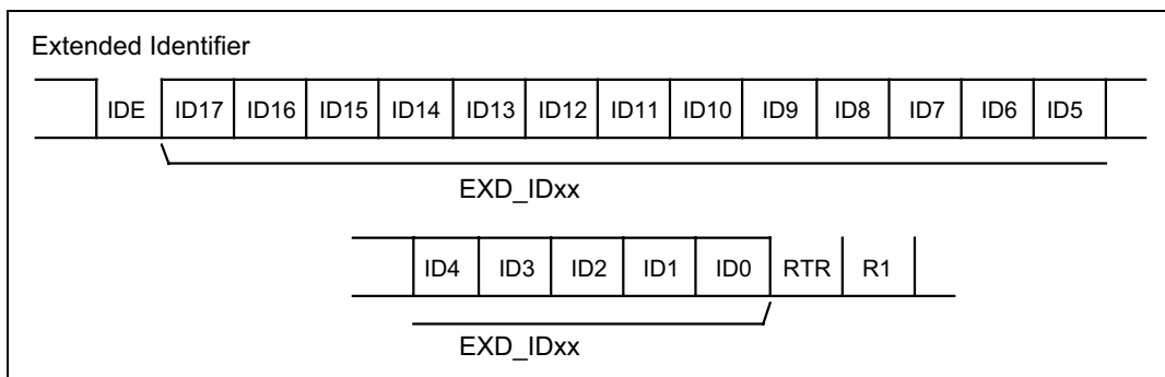
Figure 16-3 Extended identifier
