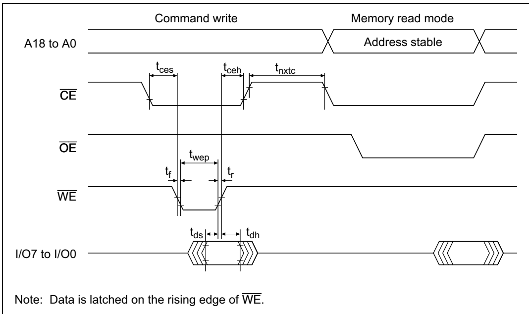
Figure 21A-18 Timing Waveforms for Memory Read after Memory Write
