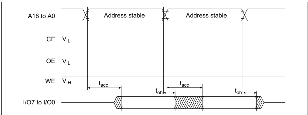
Figure 21C-20 \overline{\text{CE}} and \overline{\text{OE}} Enable State Read Timing Waveforms
