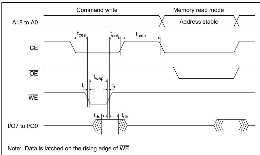
Figure 21B-18 Timing Waveforms for Memory Read after Memory Write
