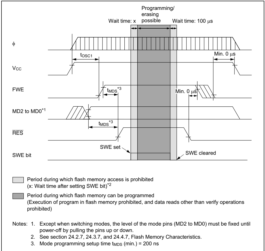
Figure 21C-26 Power-On/Off Timing (Boot Mode)
