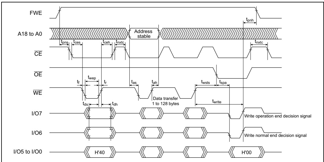
Figure 21A-22 Auto-Program Mode Timing Waveforms
