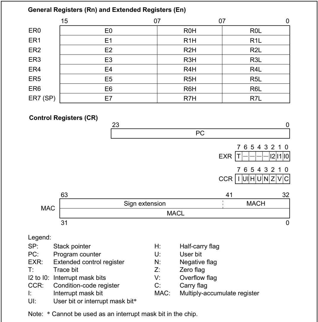
Figure 2-7 CPU Registers
