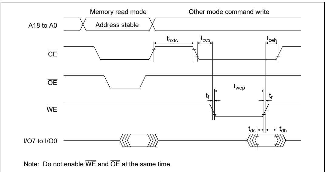
Figure 21C-19 Timing Waveforms in Transition from Memory Read Mode to Another Mode
