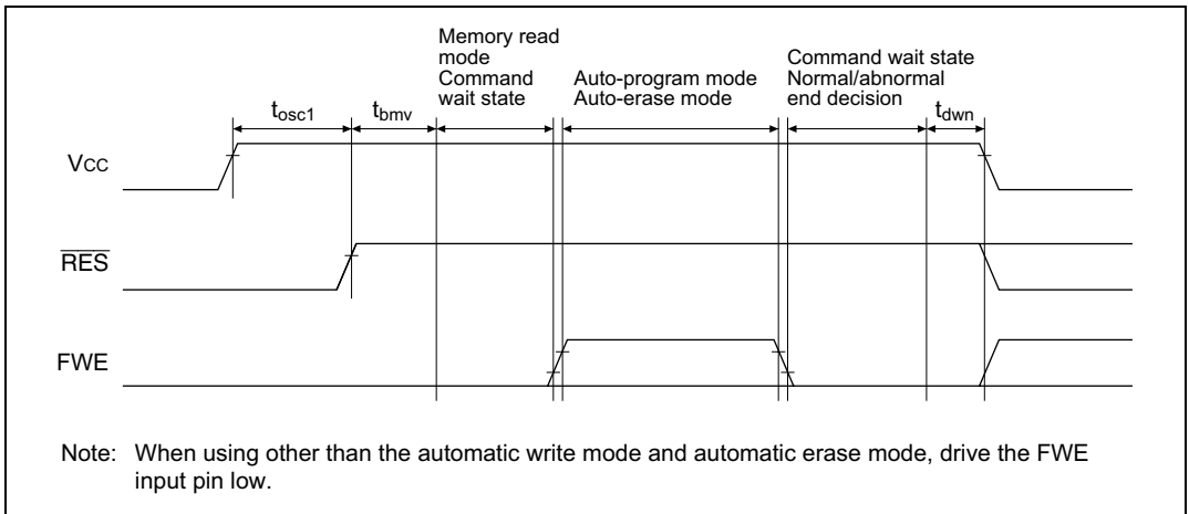
Figure 21C-25 Oscillation Stabilization Time, Boot Program Transfer Time, and Power-Down Sequence
