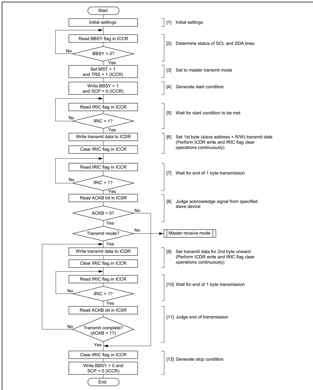
Figure 15-7 Flowchart for Master Transmit Mode (Example)
