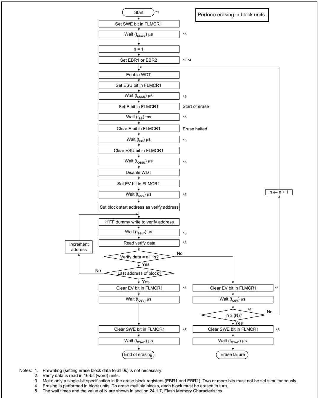
Figure 21A-13 Erase/Erase-Verify Flowchart
