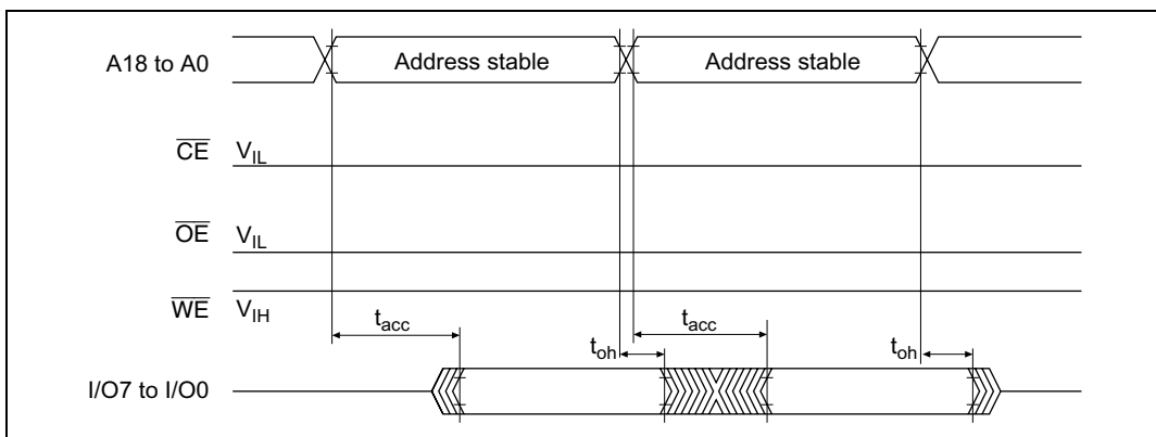
Figure 21B-20 \overline{\text{CE}} and \overline{\text{OE}} Enable State Read Timing Waveforms
