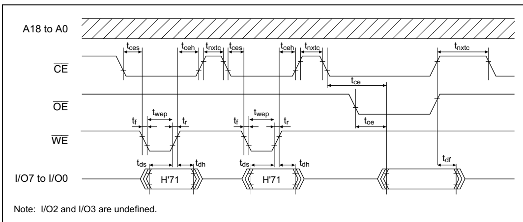
Figure 21C-24 Status Read Mode Timing Waveforms
