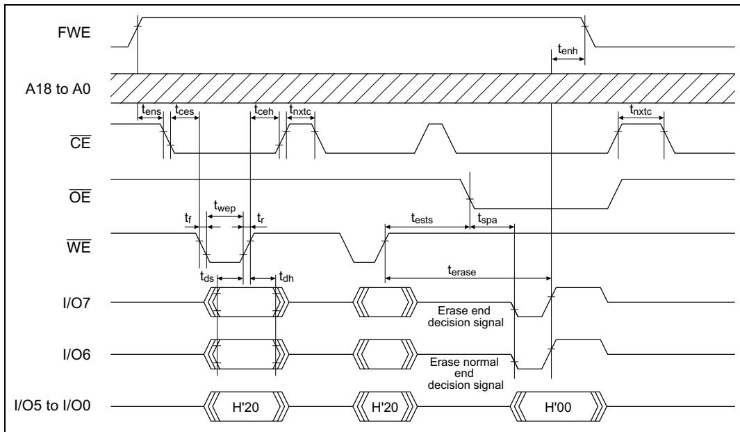
Figure 21B-23 Auto-Erase Mode Timing Waveforms
