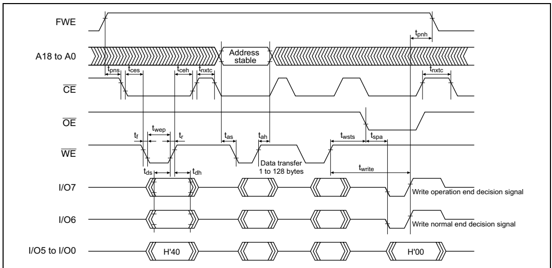
Figure 21C-22 Auto-Program Mode Timing Waveforms
