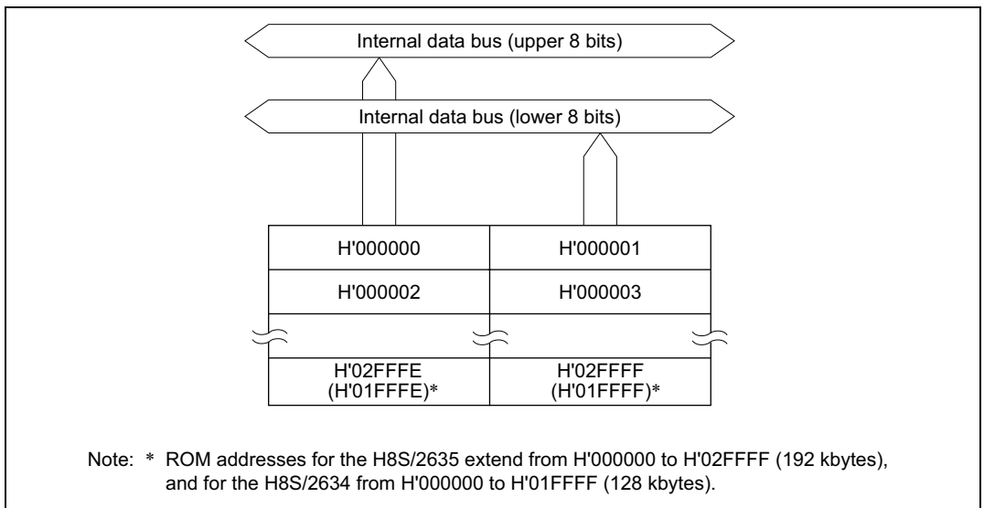
Figure 21C-1 Block Diagram of ROM 192 kbytes (128 kbytes)*
