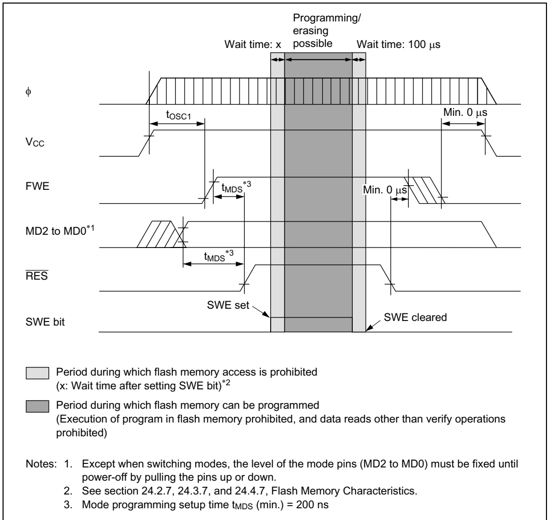
Figure 21B-26 Power-On/Off Timing (Boot Mode)
