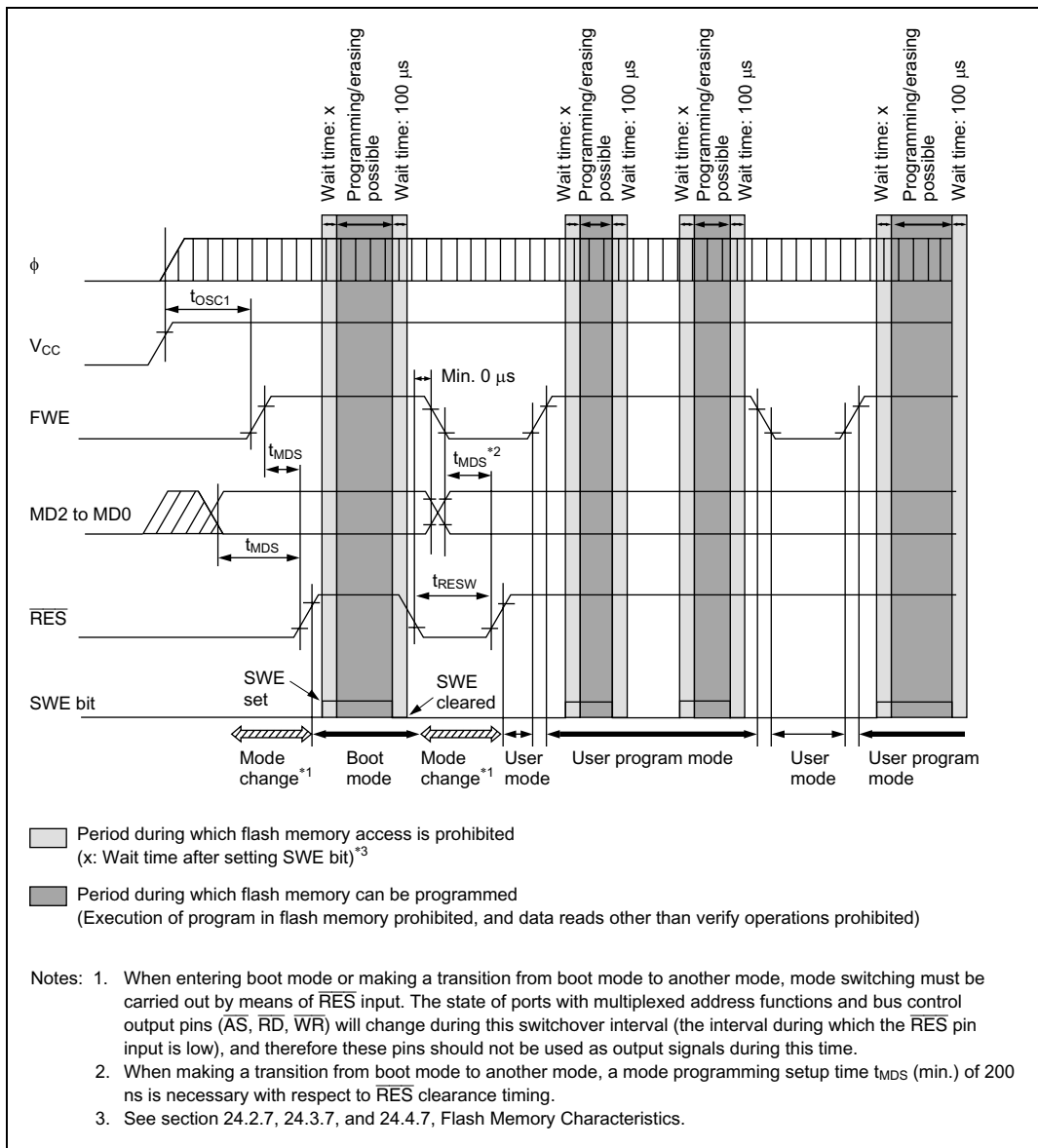
Figure 21B-28 Mode Transition Timing (Example: Boot Mode → User Mode ↔ User Program Mode)
