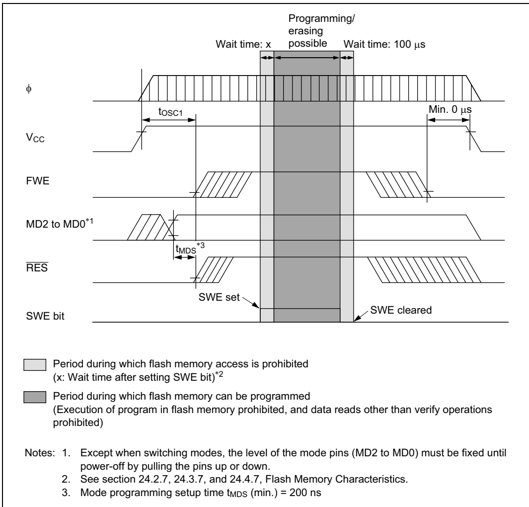
Figure 21C-27 Power-On/Off Timing (User Program Mode)
