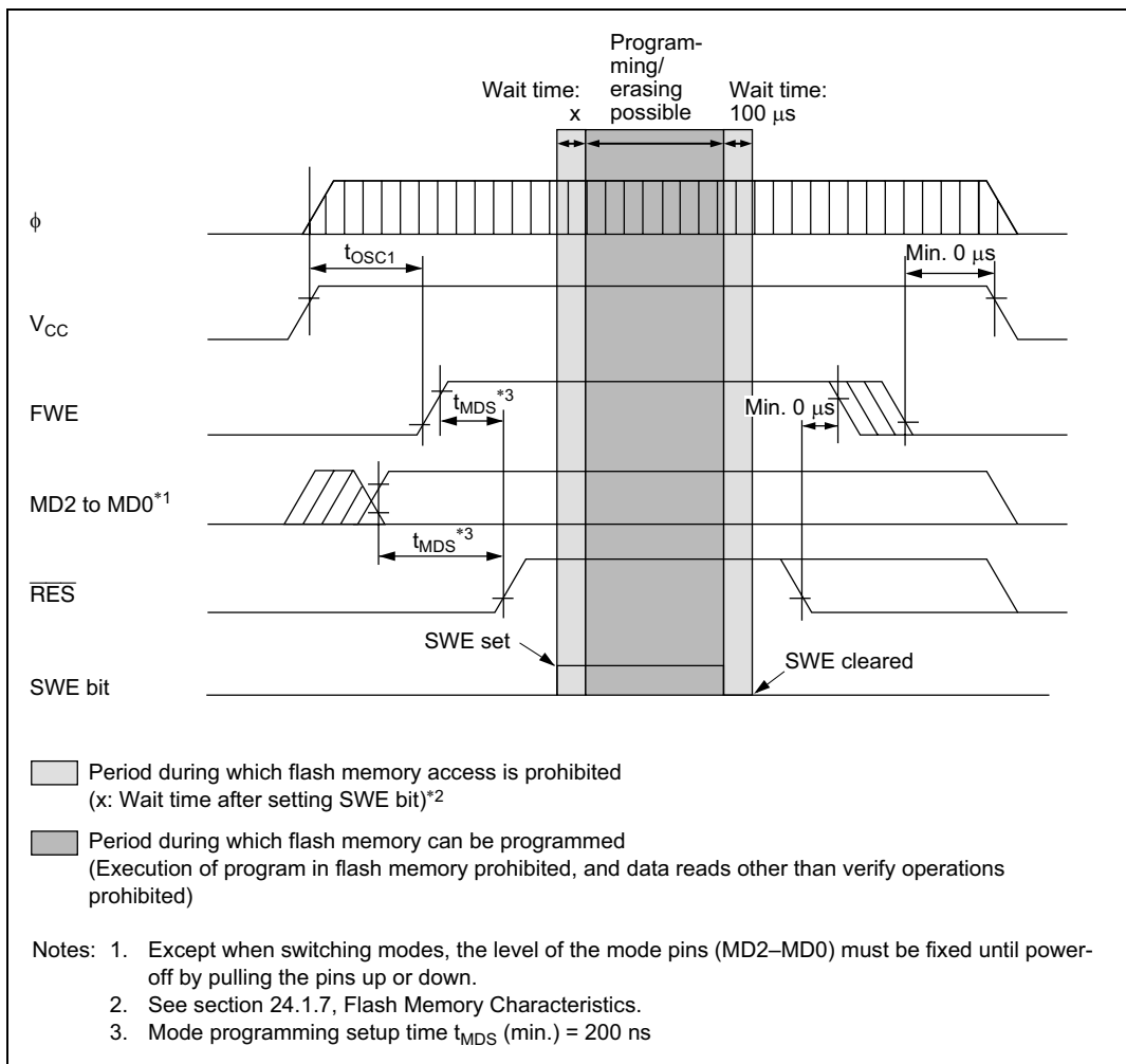
Figure 21A-26 Power-On/Off Timing (Boot Mode)
