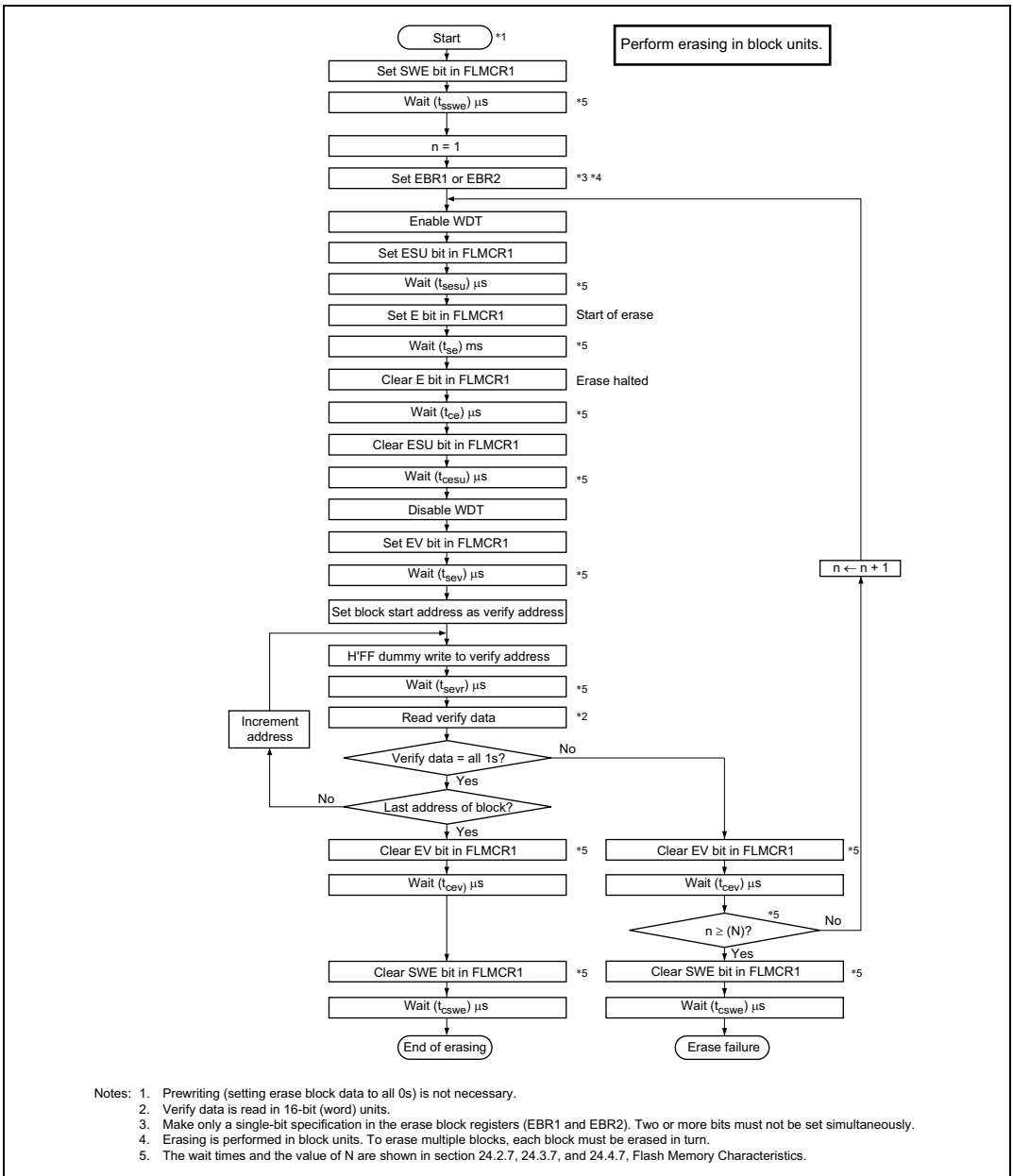
Figure 21C-13 Erase/Eraser-Verify Flowchart
