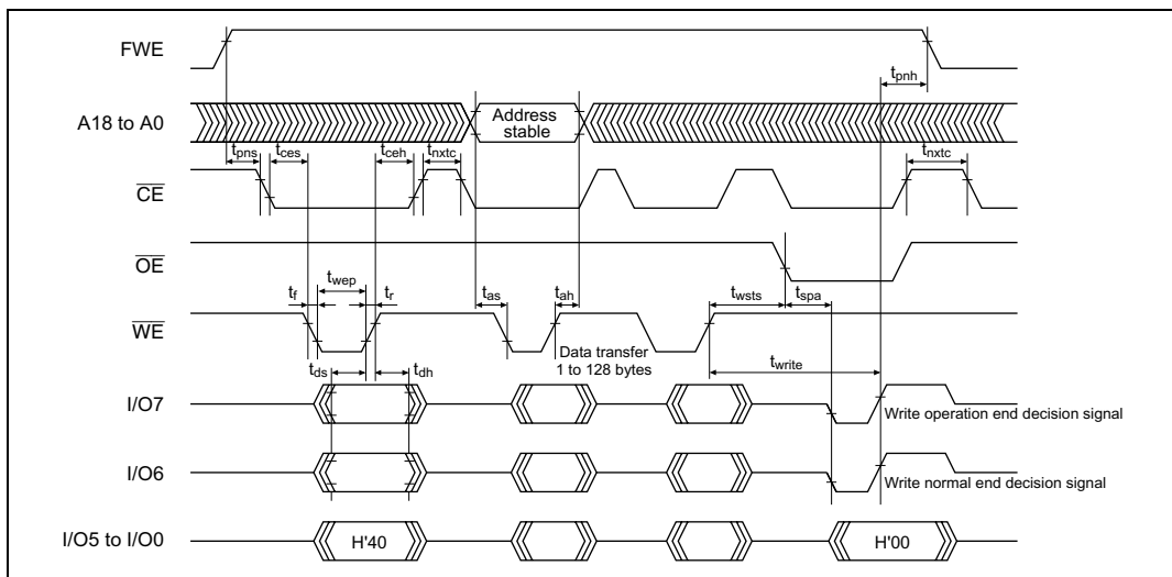
Figure 21B-22 Auto-Program Mode Timing Waveforms
