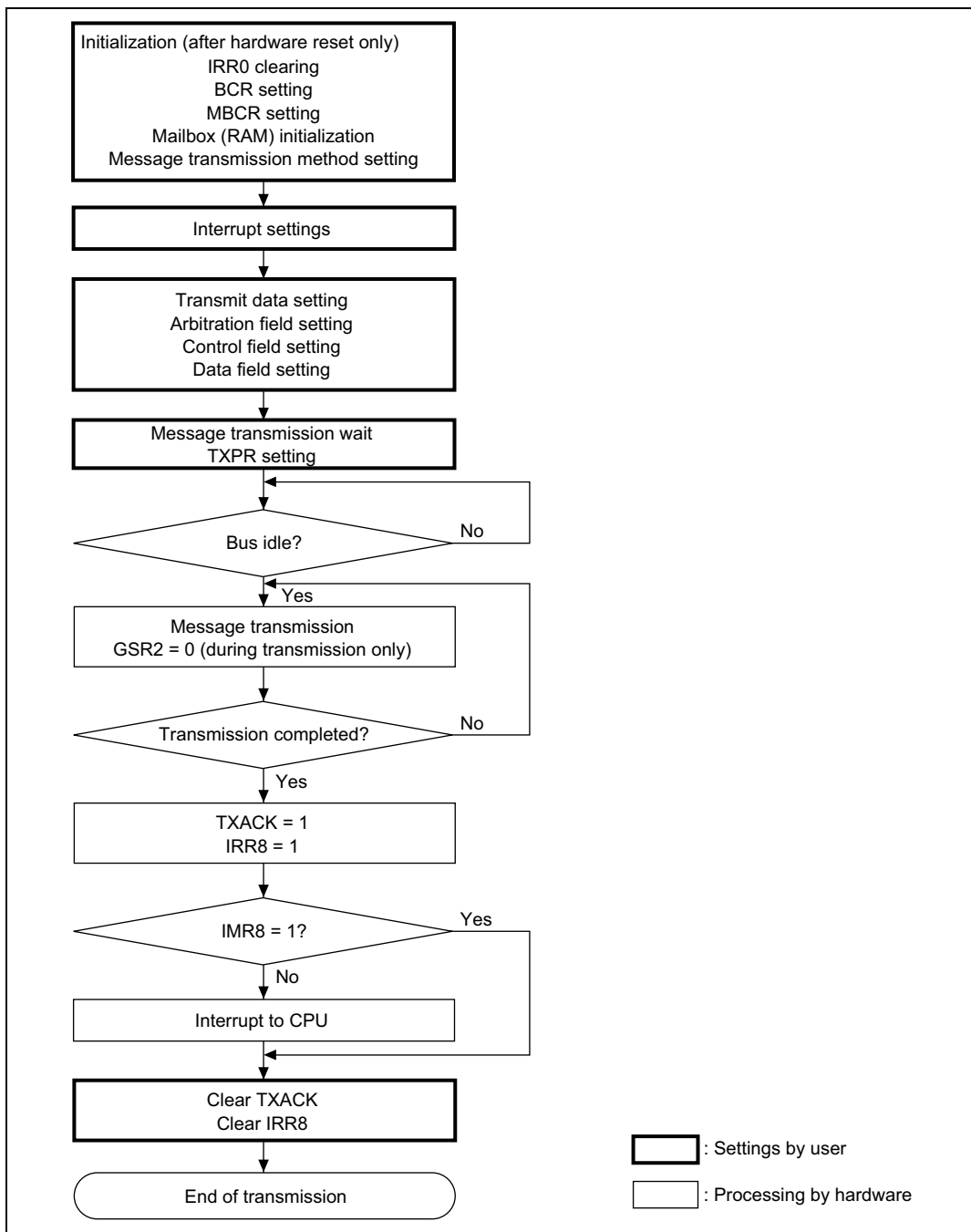
Figure 16-7 Transmission Flowchart
