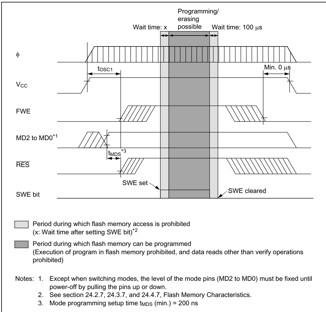
Figure 21B-27 Power-On/Off Timing (User Program Mode)
