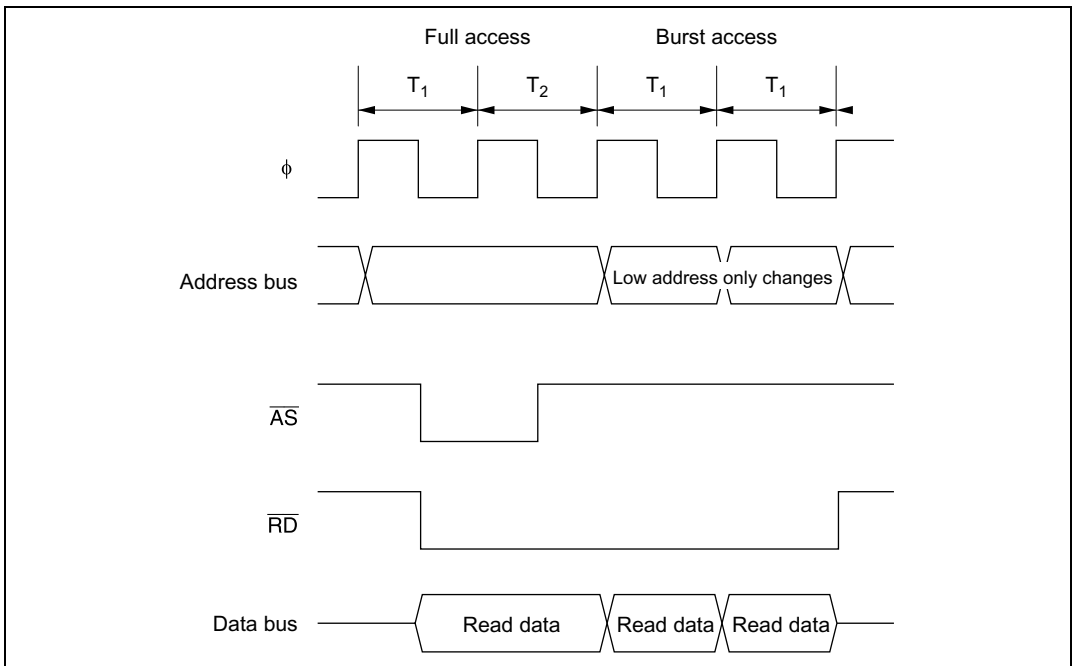
Figure 7-14 (b) Example Burst ROM Access Timing ( AST0 = BRSTS1 = 0 )
