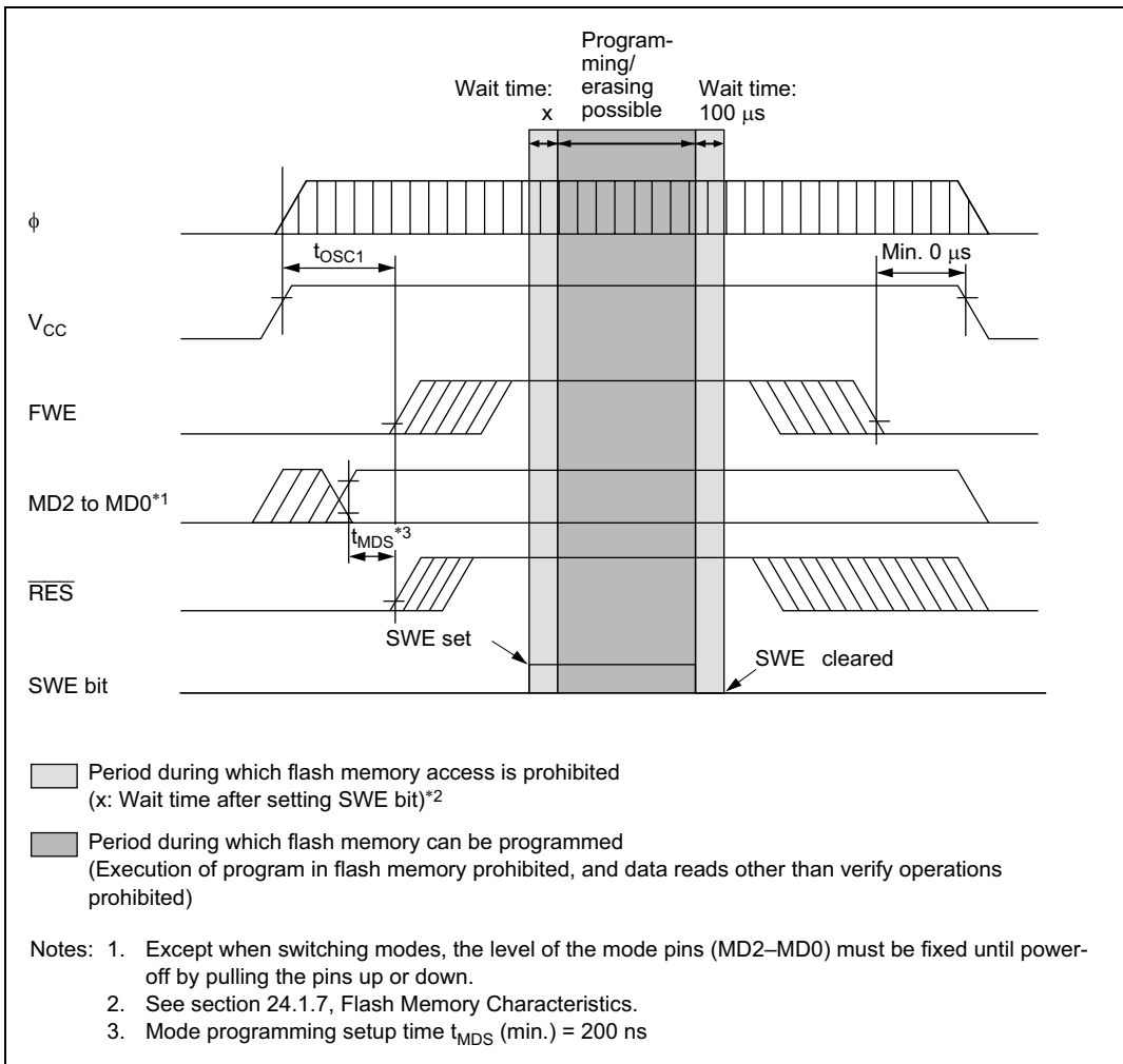
Figure 21A-27 Power-On/Off Timing (User Program Mode)
