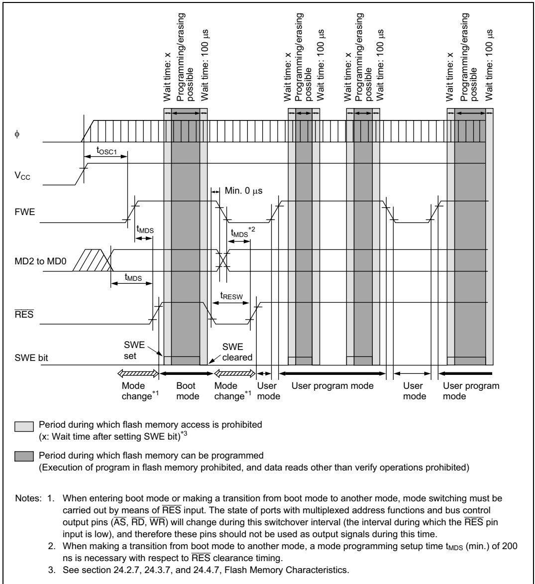
Figure 21C-28 Mode Transition Timing (Example: Boot Mode → User Mode ↔ User Program Mode)
