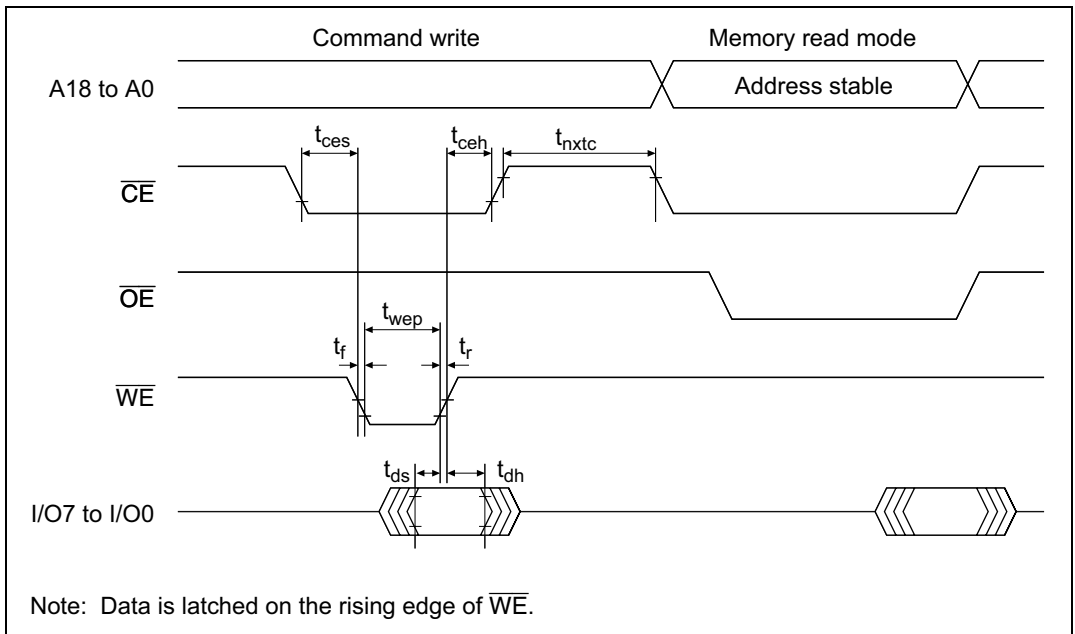
Figure 21C-18 Timing Waveforms for Memory Read after Memory Write
