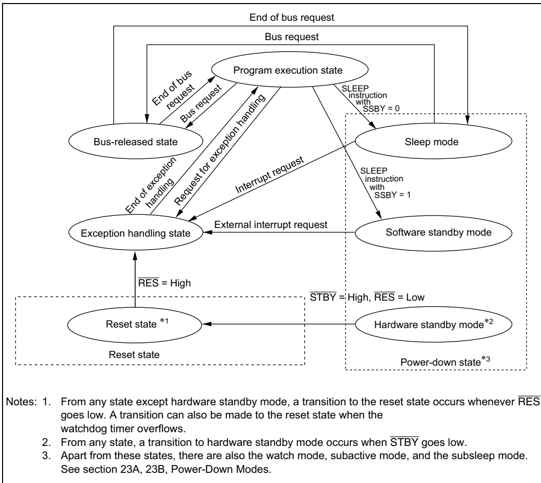
Figure 2-15 State Transitions
