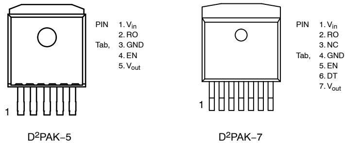
Figure 3. Pin Connections
