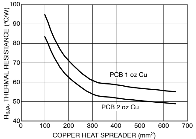
Figure 25. Thermal Resistance vs. PCB Copper Area (D2PAK-5)
