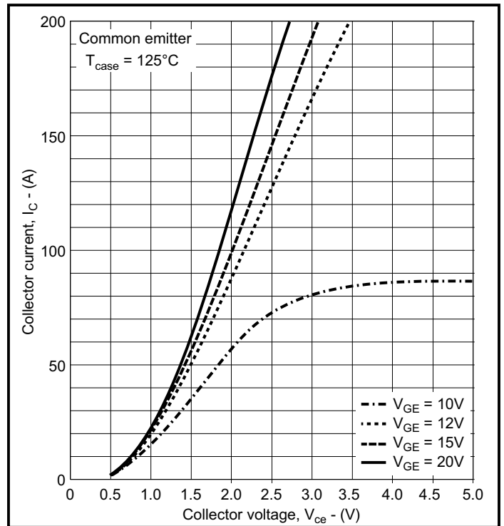
Fig. 4 Typical output characteristics DataSheet4U.com
