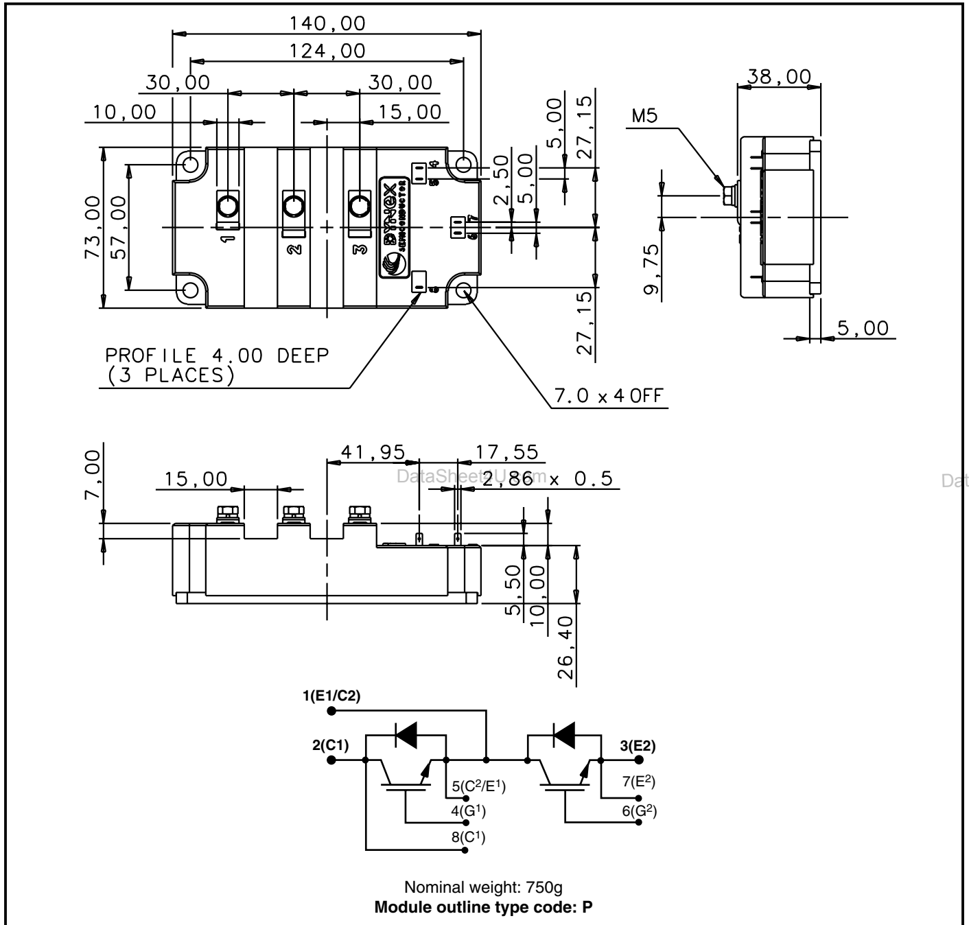
Fig. 11 Package details
