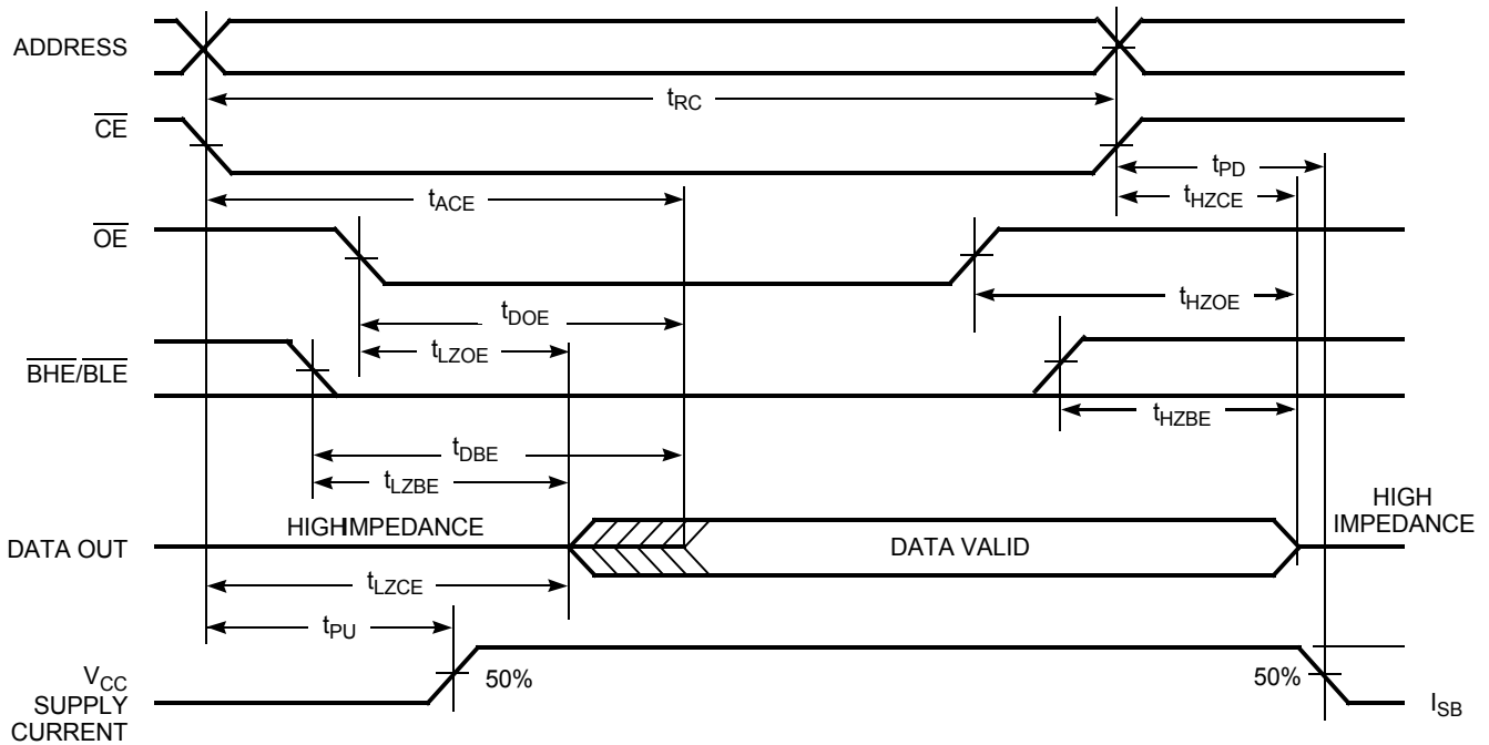
Figure 6. Read Cycle No. 2 ( \overline{OE} Controlled) [16, 17]
