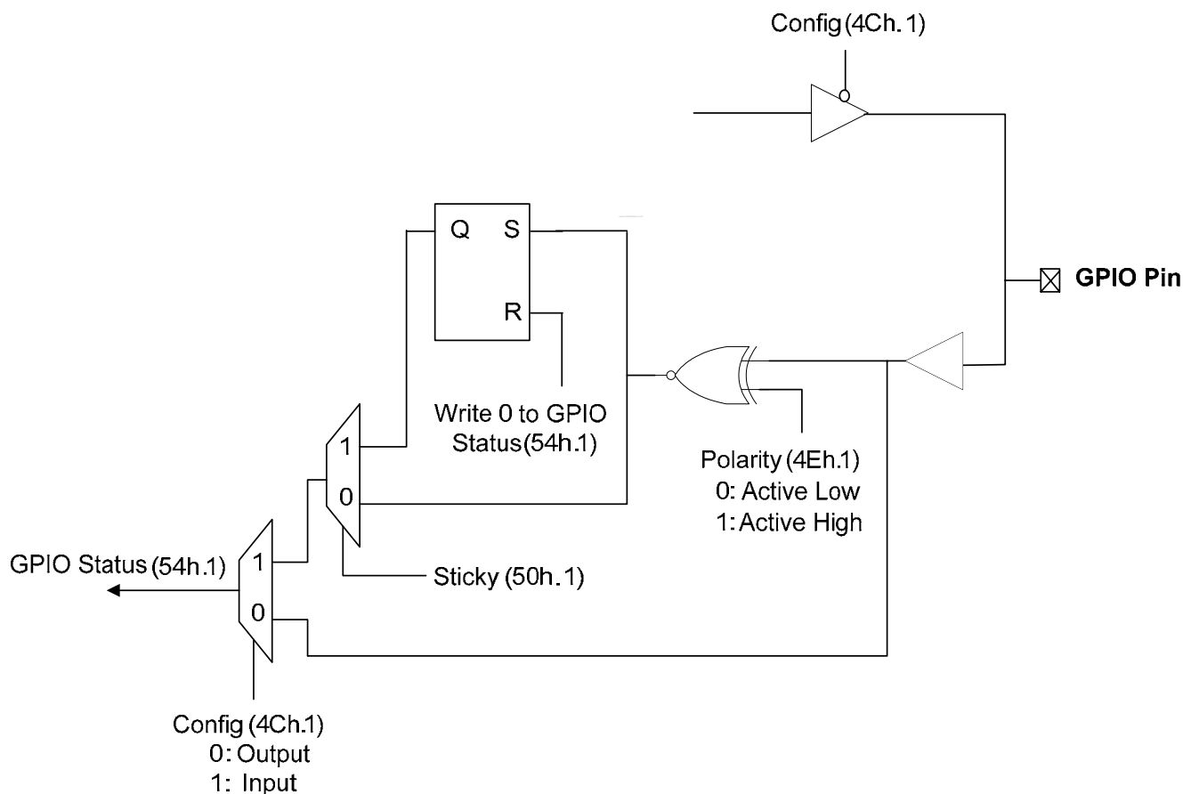
Figure 18. GPIO Implementation
