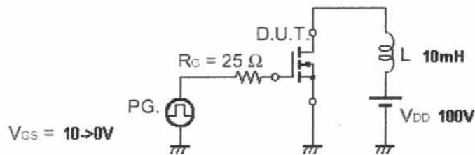
Test Circuit – Avalanche Capability
