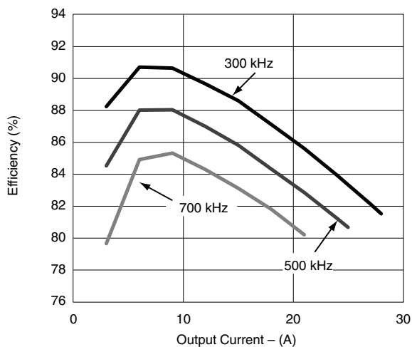
Figure 2. Total Efficiency 12 V IN /1.3 V OUT
