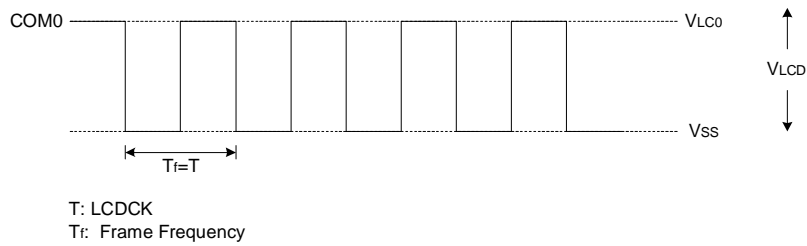
Figure 13. LCD Common Signal Waveform (static)
