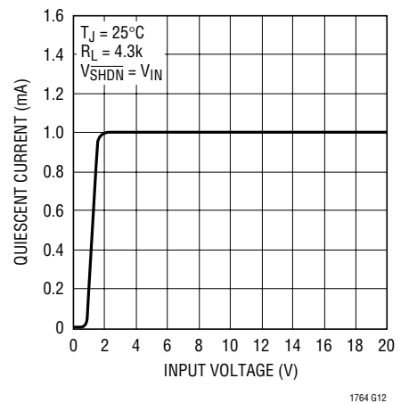
LT1764 Quiescent Current
