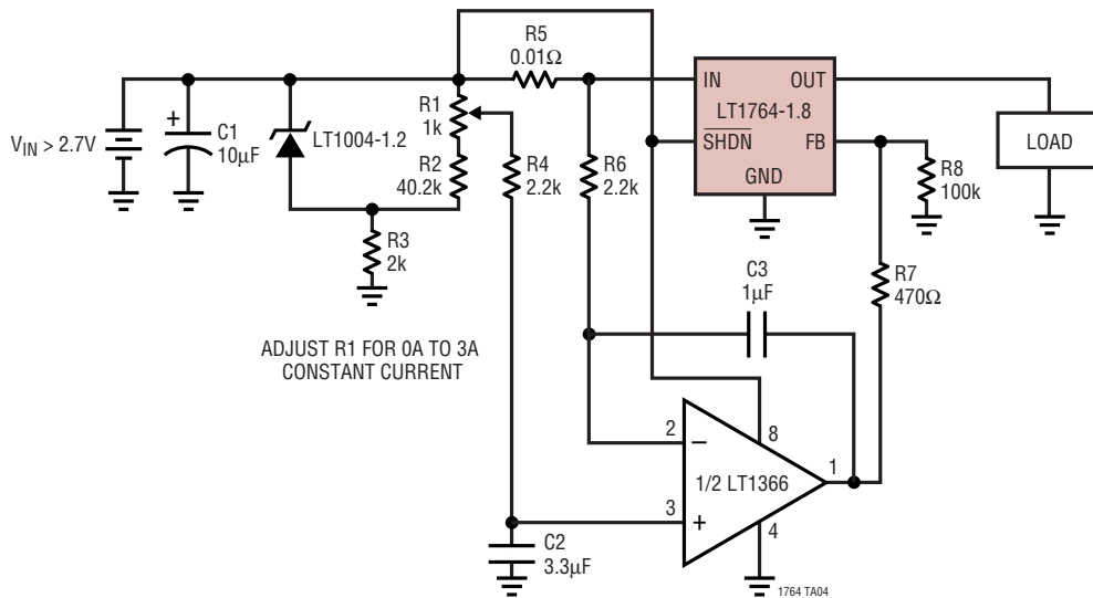
Adjustable Current Source
