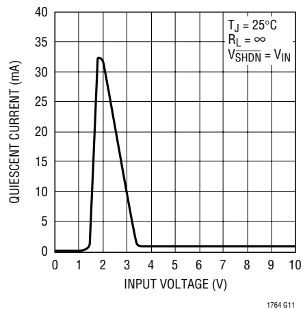
LT1764-3.3 Quiescent Current
