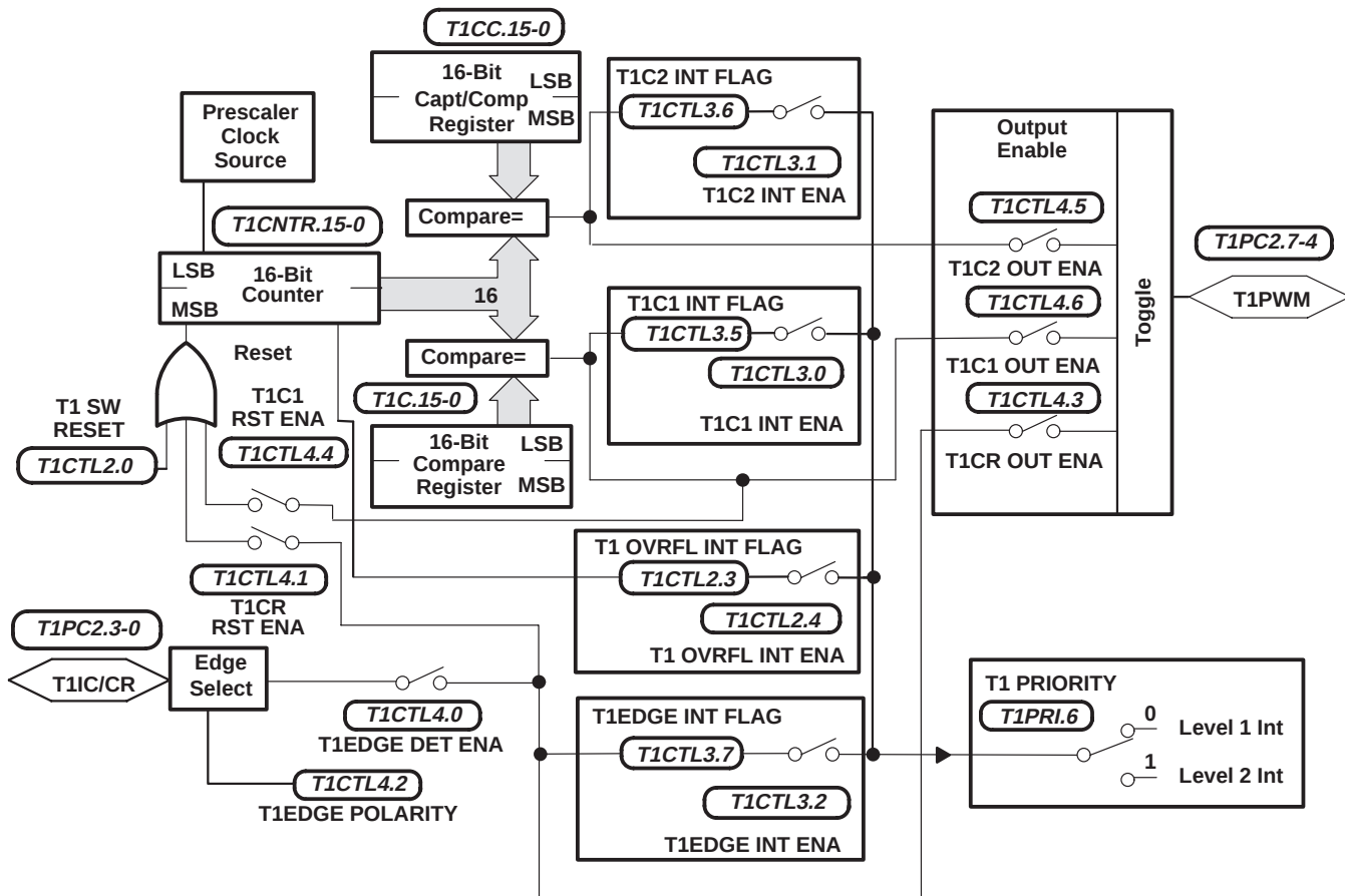
Figure 7. Dual-Compare Mode
