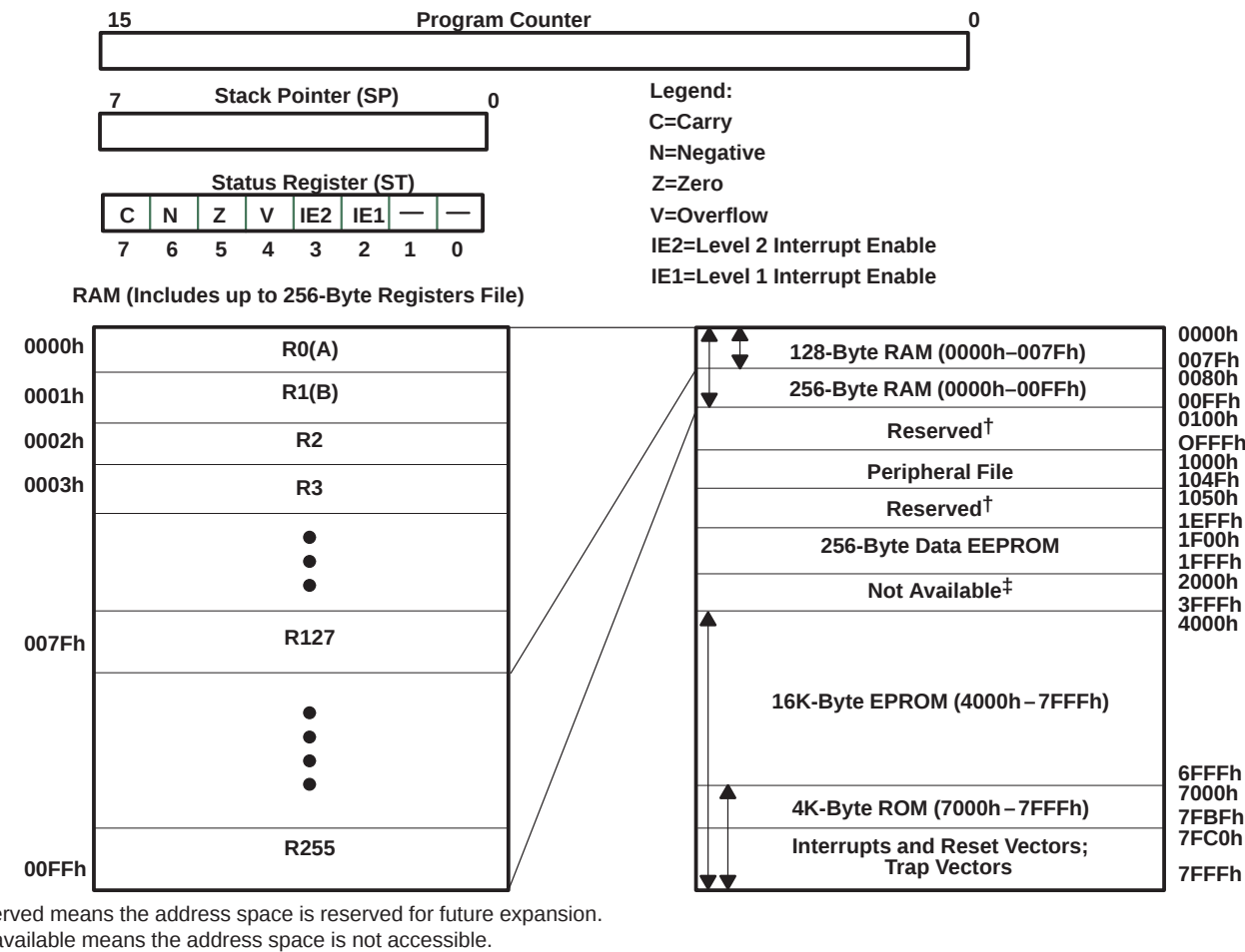
Figure 1. Programmer's Model
