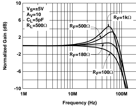
Non-Inverting Frequency Response for Various R_F
