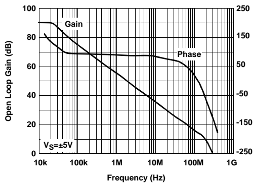
Open Loop Gain/Phase
