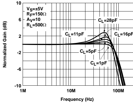
Non-Inverting Frequency Response for Various C_L
