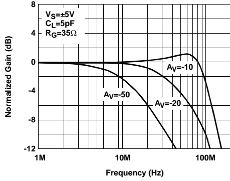
Inverting Frequency Response for Various Gain
