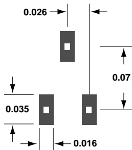
Figure 32. PCB Pad Layout (dimensions in inches).
