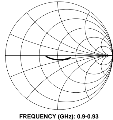
Figure 15. Input Impedance.
