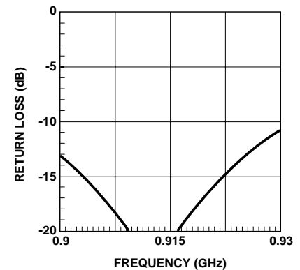
Figure 16. Input Return Loss.
