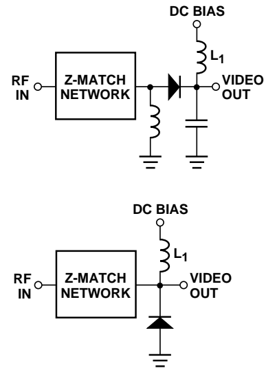
Figure 12. Basic Detector Circuits.
