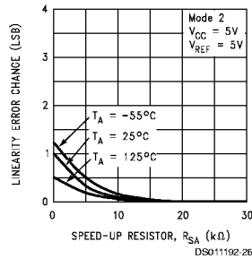
Linearity Change vs Speed-Up Resistor
