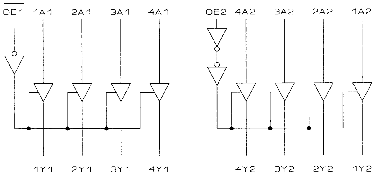
FIGURE 3. Logic diagram.
