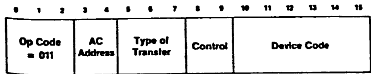
Fig. 7 Input/Output Instruction Fields
