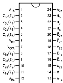
24-Pin DIP
