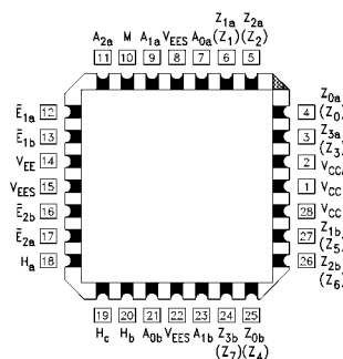
28-Pin PLCC
