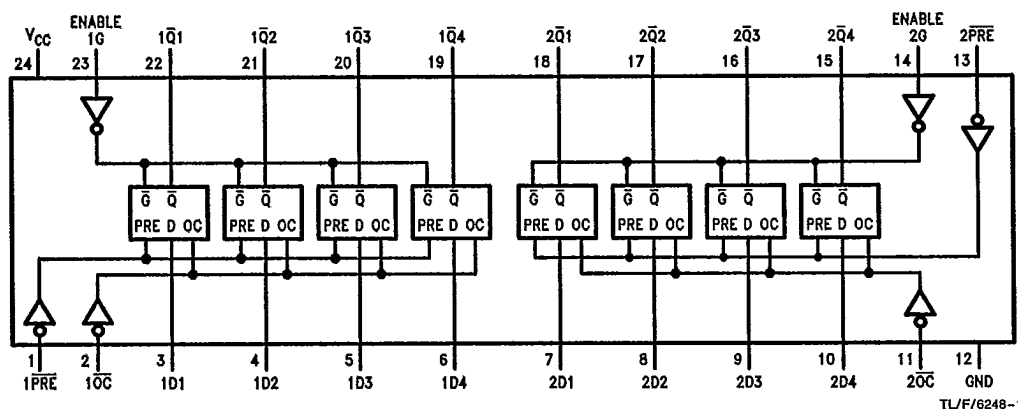
Dual-In-Line Package
