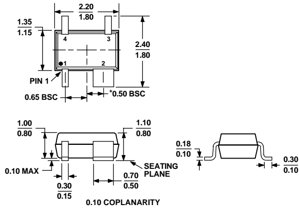
Figure 21. 4-Lead Thin Shrink Small Outline Transistor Package [SC70] (EIAJ SC82 body) (KS-4)
