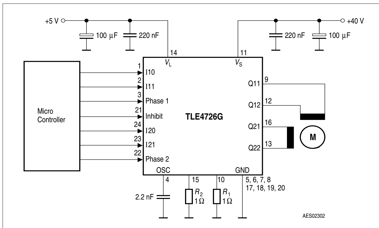
Figure 4 Application Circuit
