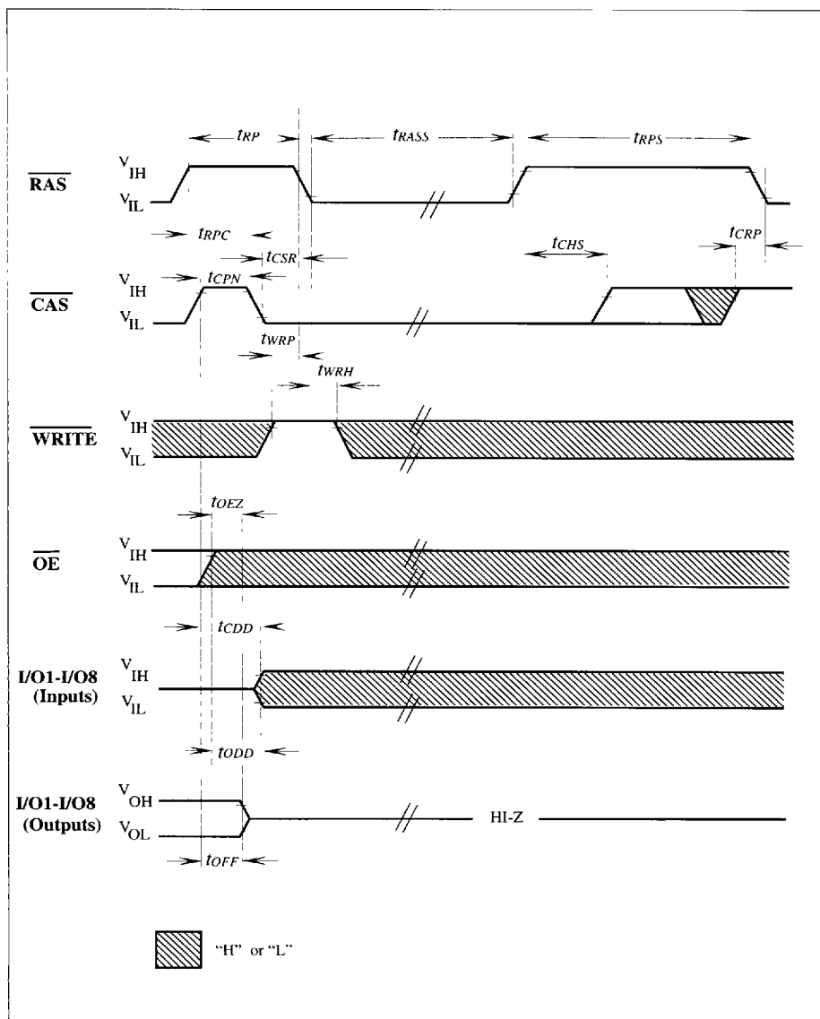
CAS before \overline{\text{RAS}} Self Refresh Cycle
