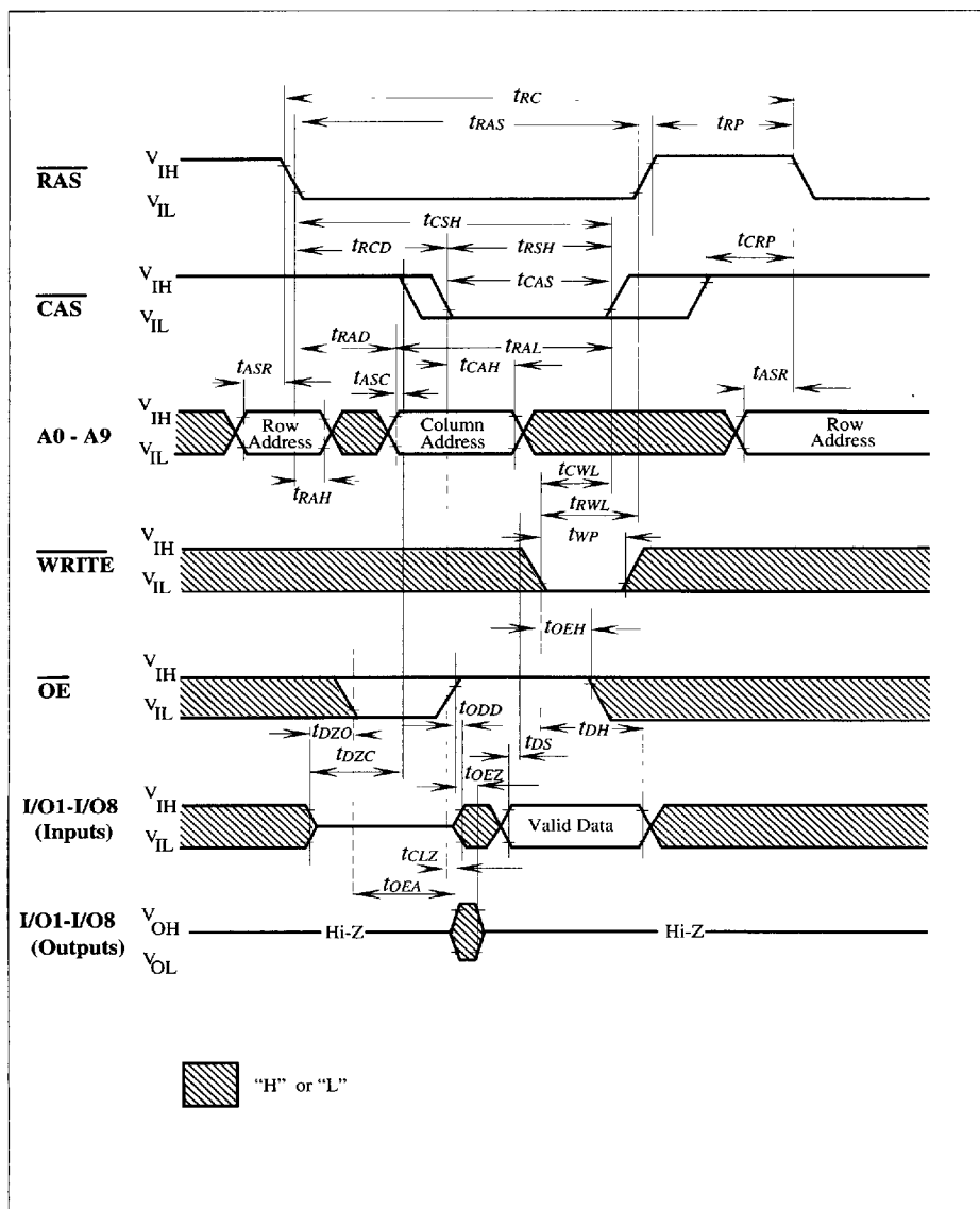
Write Cycle ( \overline{\text{OE}} Controlled Write)
