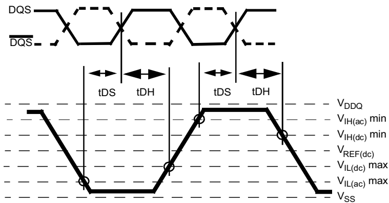
Differential input waveform timing - t_{DS} and t_{DH}
