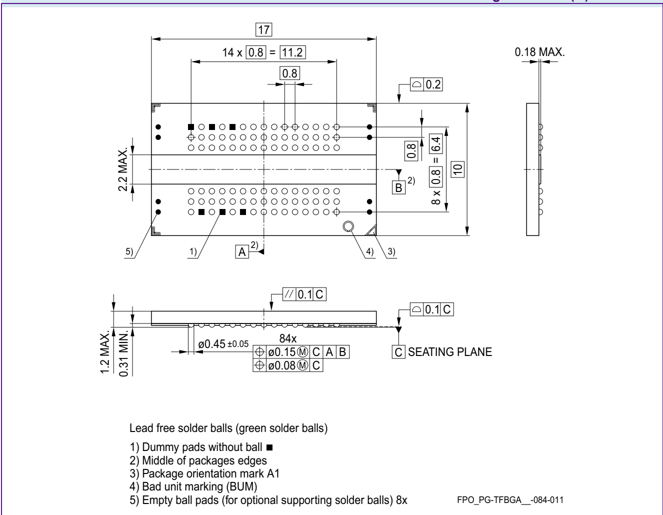
FIGURE 11 Package Outline P(G)-TFBGA-84
