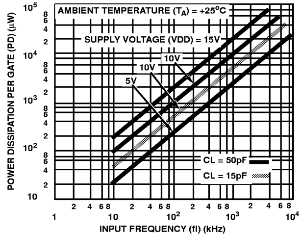
FIGURE 2. TYPICAL POWER DISSIPATION vs FREQUENCY
