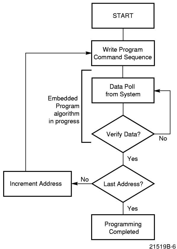
Figure 3. Program Operation
