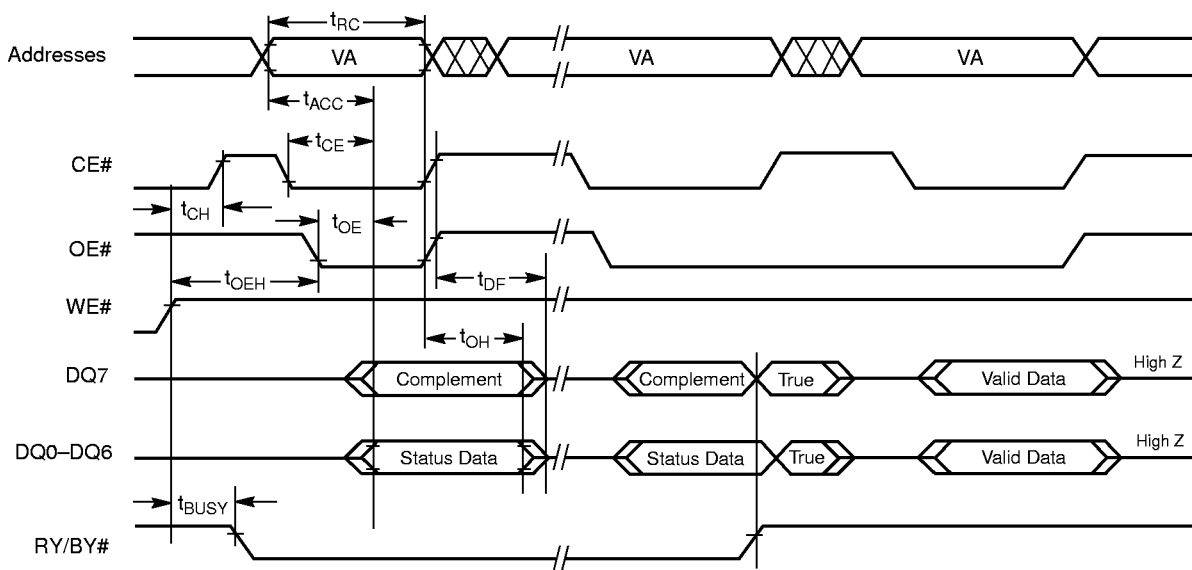
Figure 19. Back-to-Back Read/Write Cycle Timings
