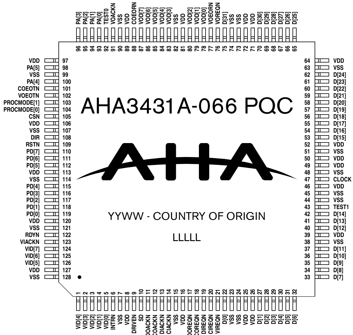
Figure 16: Pinout
