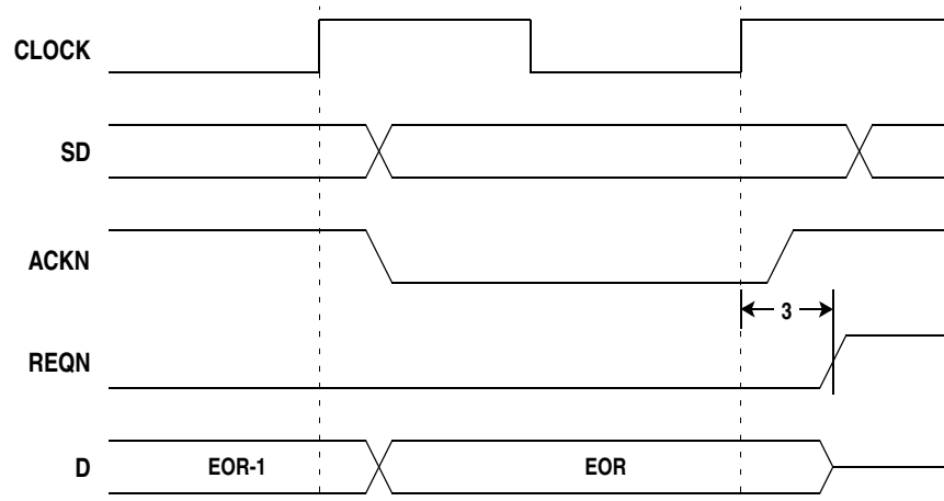
Figure 20: Request Deasserts at EOR, Strobe Condition of DSC=0-3, 6-7; ERC=1
