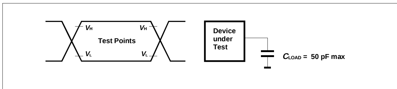
Figure 7-1 Input/Output Waveform for AC Measurements
