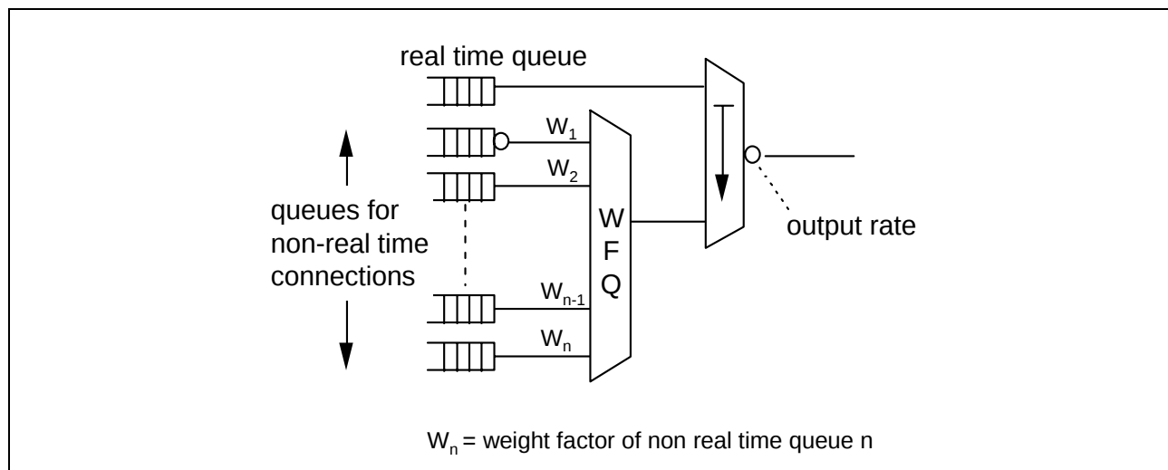
Figure 3-3 Scheduler Structure
