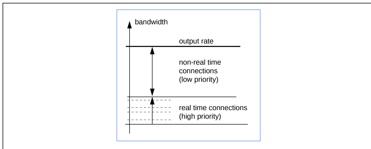
Figure 3-4 Scheduler Behavior
