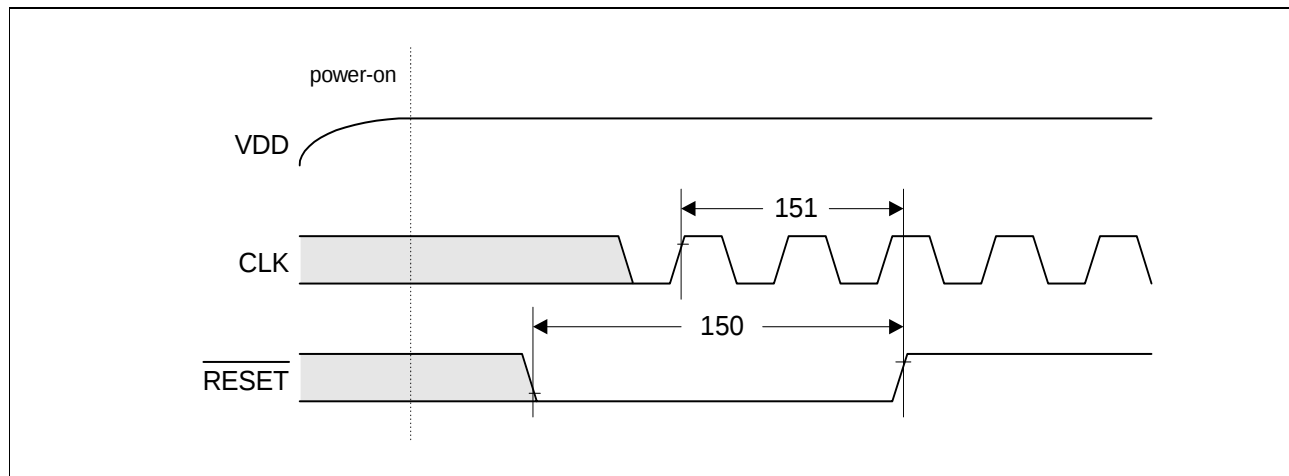
Figure 7-10 Reset Timing
