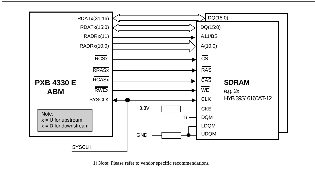
Figure 5-4 SDRAM Interfaces
