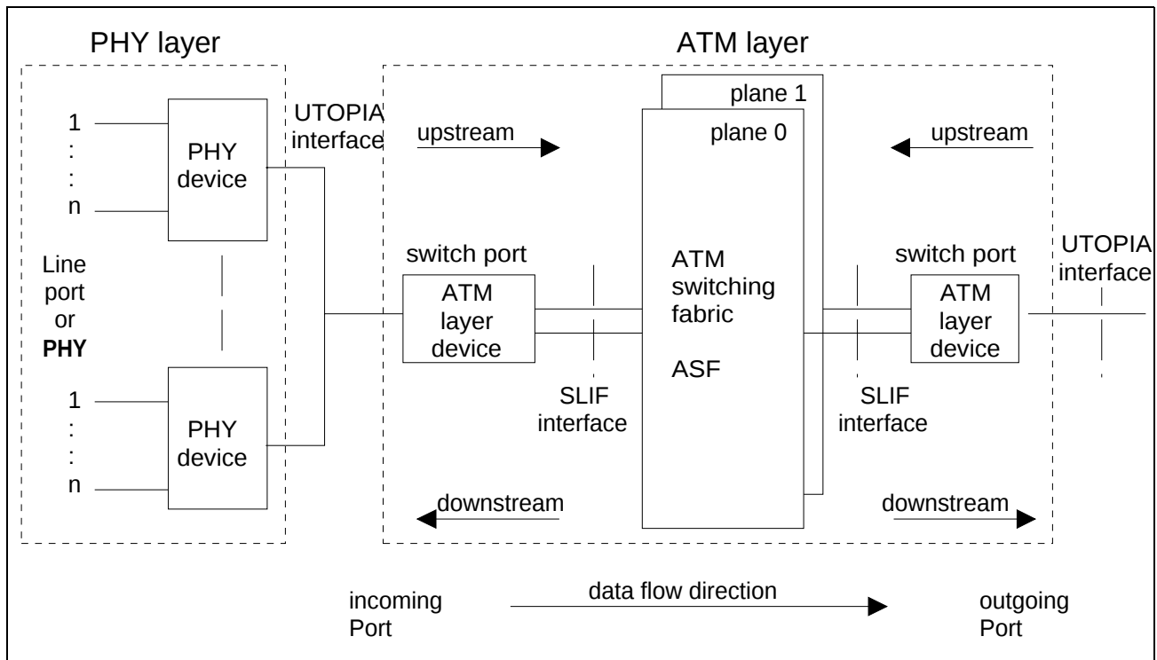
Figure 1-6 Nomenclature
