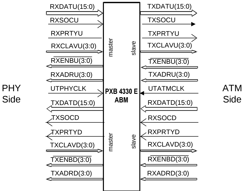
Figure 5-1 UTOPIA Interfaces
