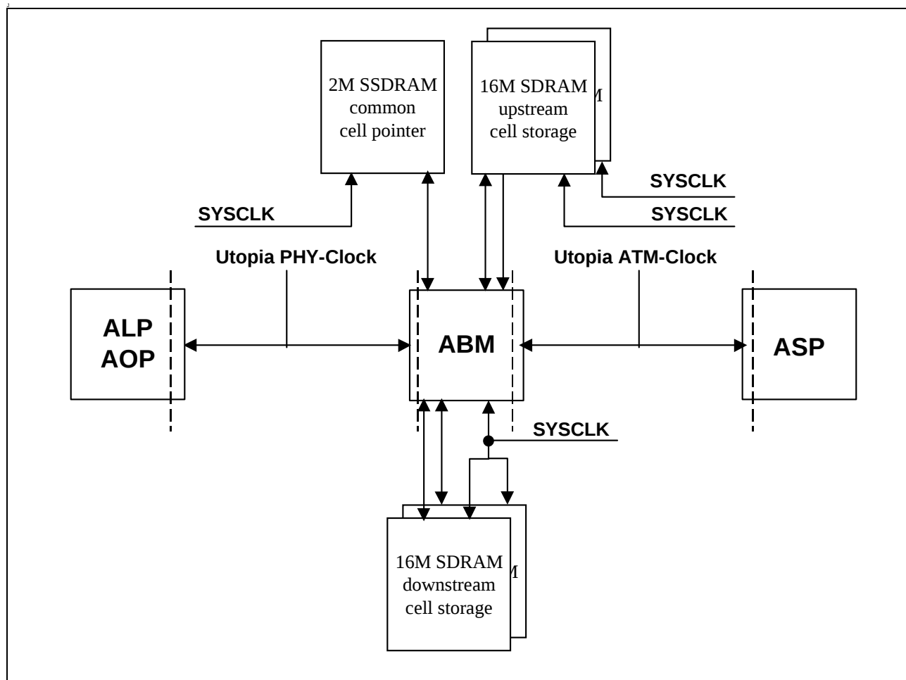
Figure 5-8 Clock Concept
