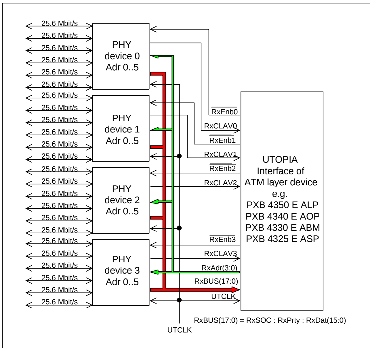
Figure 5-2 Upstream Receive UTOPIA Example: 4 x 6 PHYs
