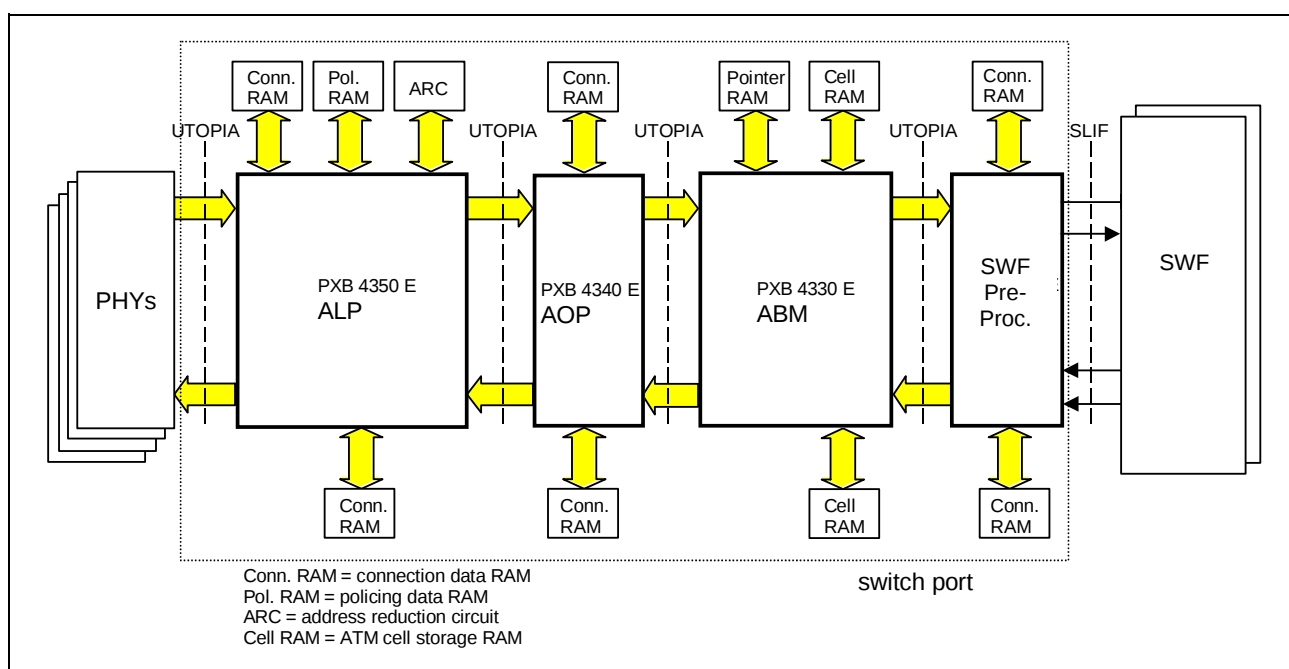
Figure 1-4 ATM Switch Basic Configuration
