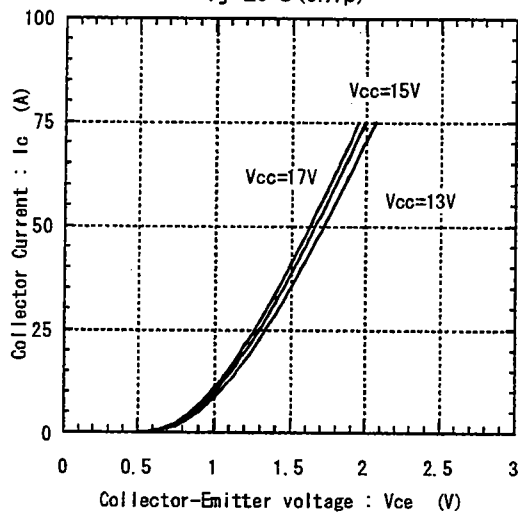
Collector current vs. Collector-Emitter voltage T_J=25^\circ\text{C} (Chip)
