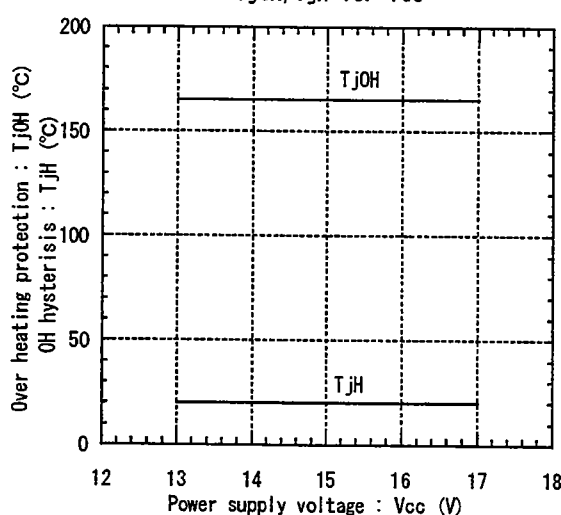
Over heating characteristics T JOH , T JH vs. V cc
