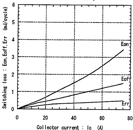
Switching Loss vs. Collector Current E_{dc}=300V, V_{cc}=15V, T_j=25^\circ C
