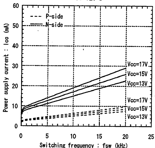
Power supply current vs. Switching frequency T c =125°C
